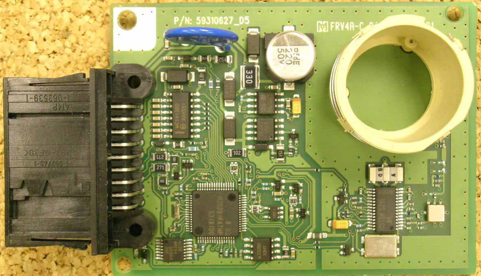
PCB (top)
