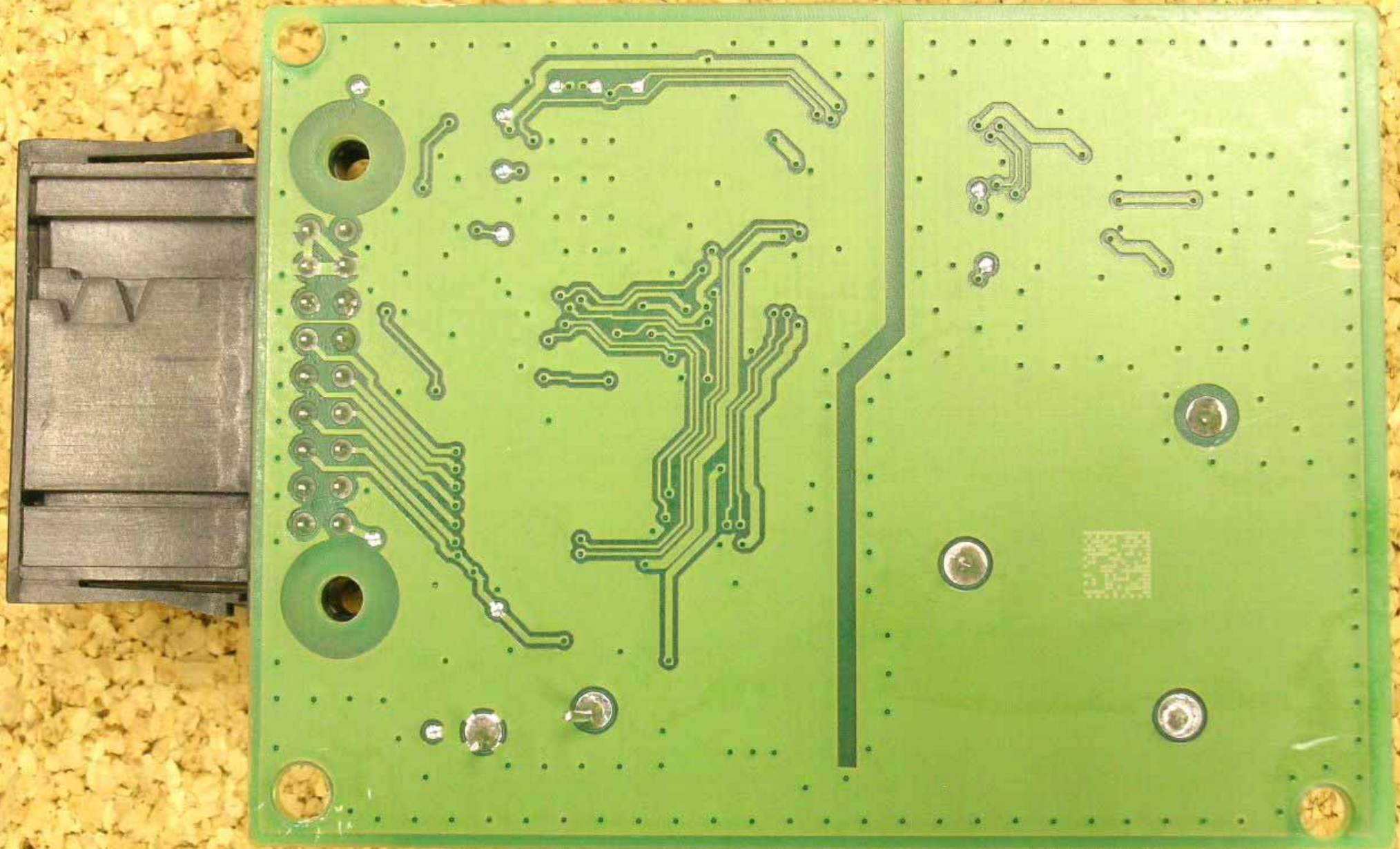
PCB (bottom)
