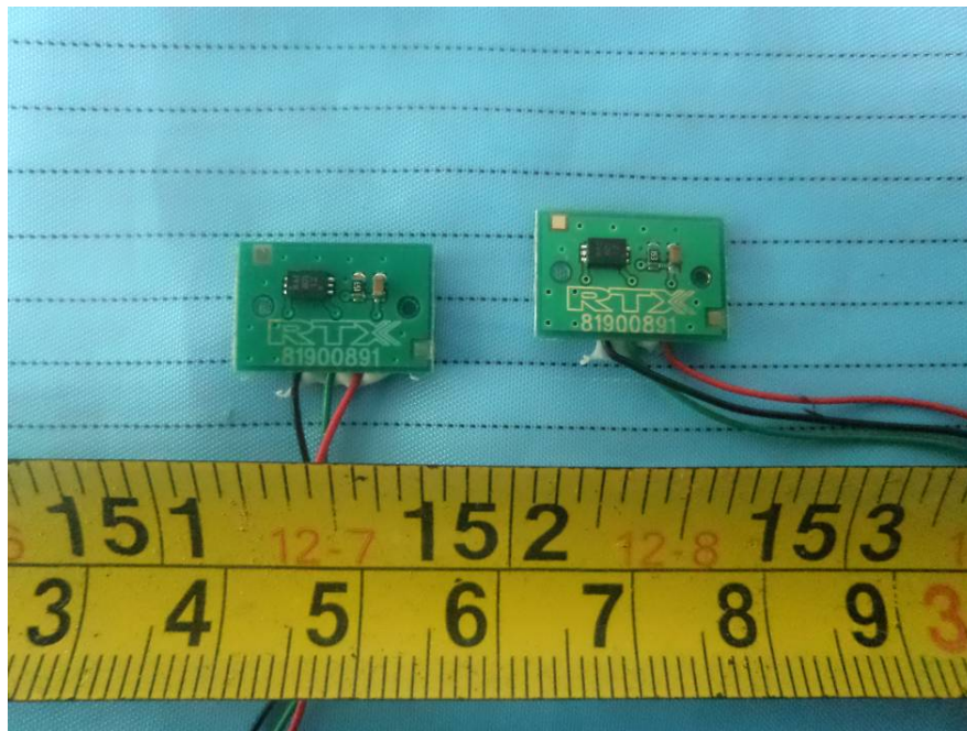
EUT – Sub-Board 1&2 Top View
