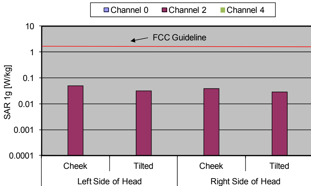
Fig. 8: The measured head phantom SAR values for the RTX Products RTX4088 for the US DECT standard in comparison to the FCC exposure limit.
