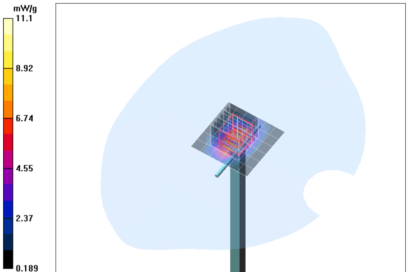
Fig. 11: Validation measurement 1900 MHz body (January 30, 2012), coarse grid. Ambient Temperature: 21.5° C, Liquid Temperature: 21.4° C.
