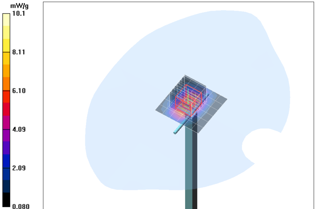
Fig. 10: Validation measurement 1900 MHz Head (January 26, 2012), coarse grid. Ambient Temperature: 22.2° C, Liquid Temperature: 21.9° C.
