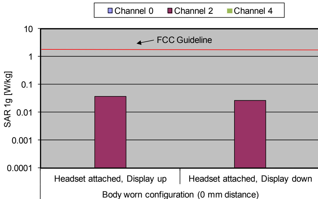
Fig. 9: The measured SAR values in body worn configuration for the RTX Products RTX4088 for the US DECT standard in comparison to the FCC exposure limit.
