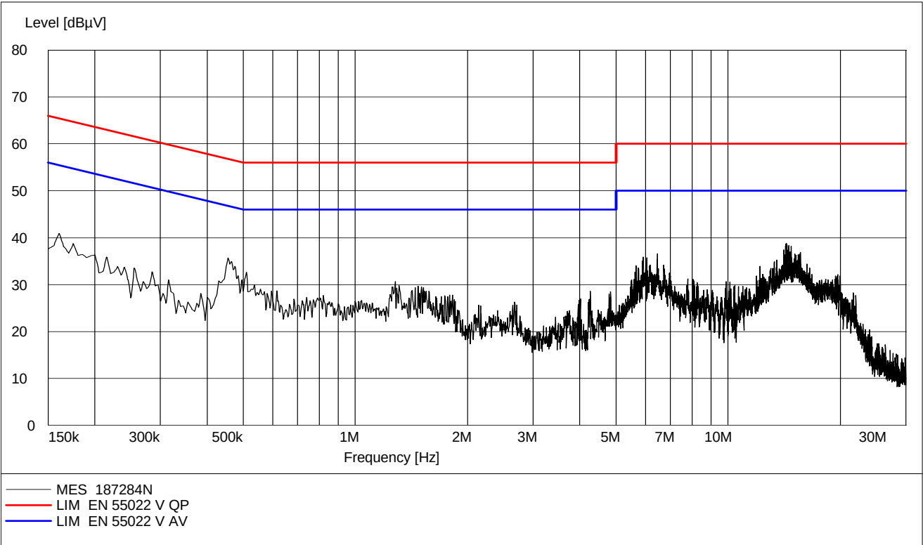
Handset Charging, Phase L1 and N, 120V 60Hz (plot shows worst case of the two phases)
