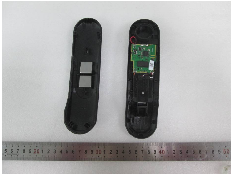
EUT 1 – Cover off View
