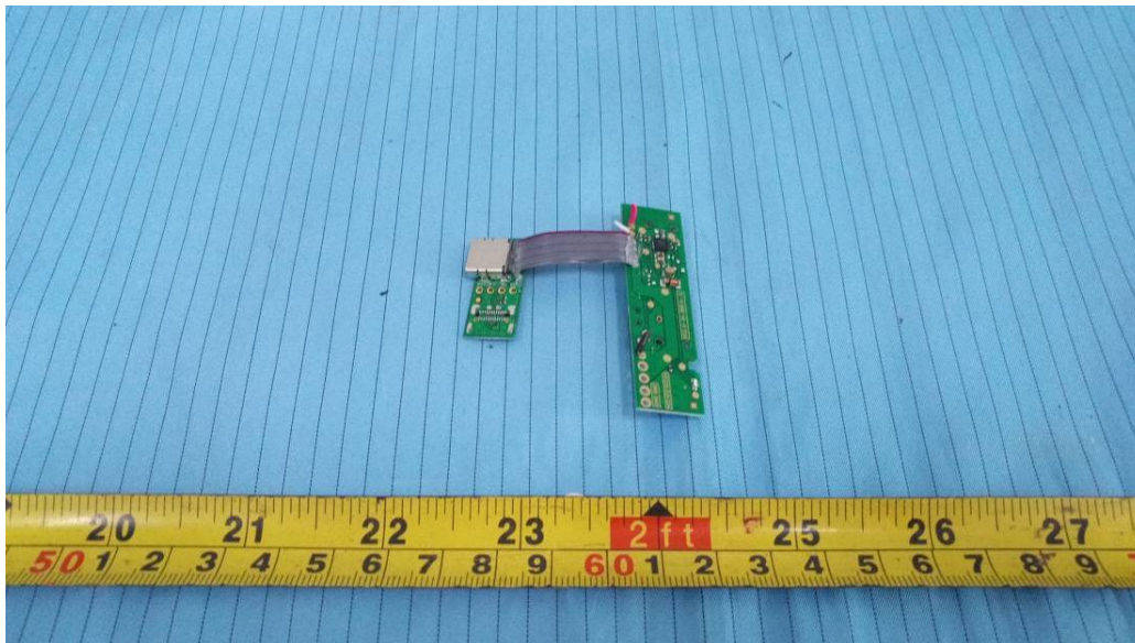
EUT(Charger 1) – Main Board Top View
