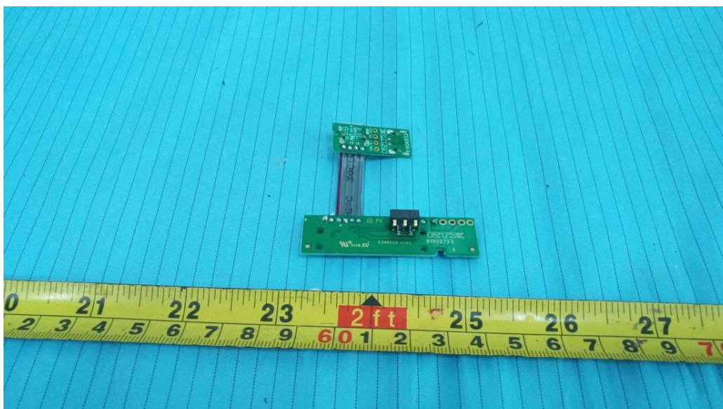
EUT(Charger 1) – Main Board Bottom View
