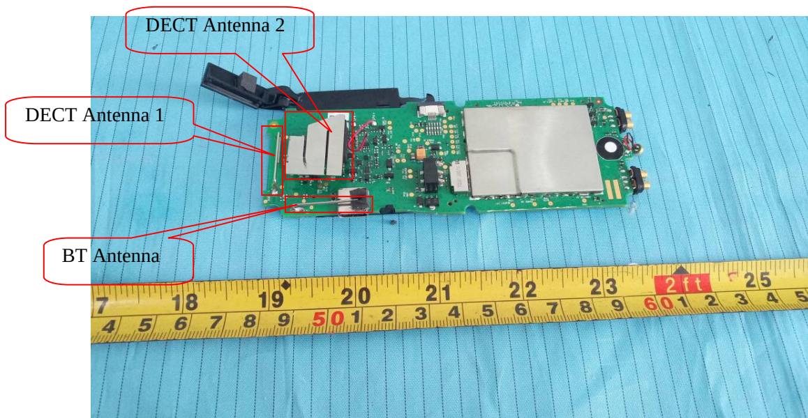
EUT – Main Board Top View 1
