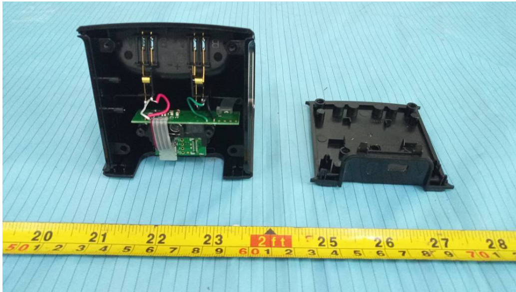
EUT(Charger 1) – Cover off View 1
