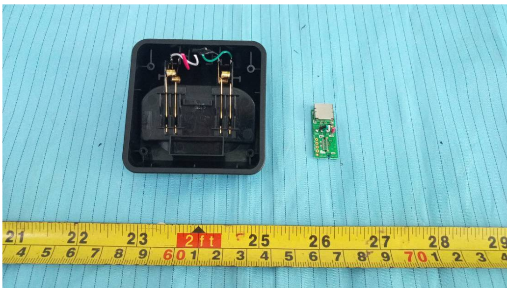
EUT(Charger 2) – Cover off View 2
