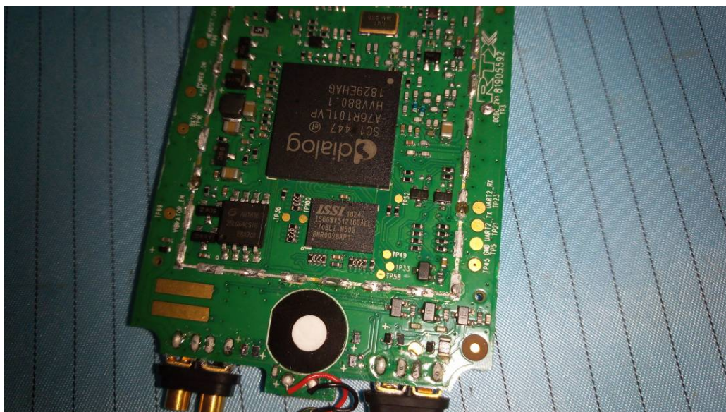
EUT – IC 2 View
