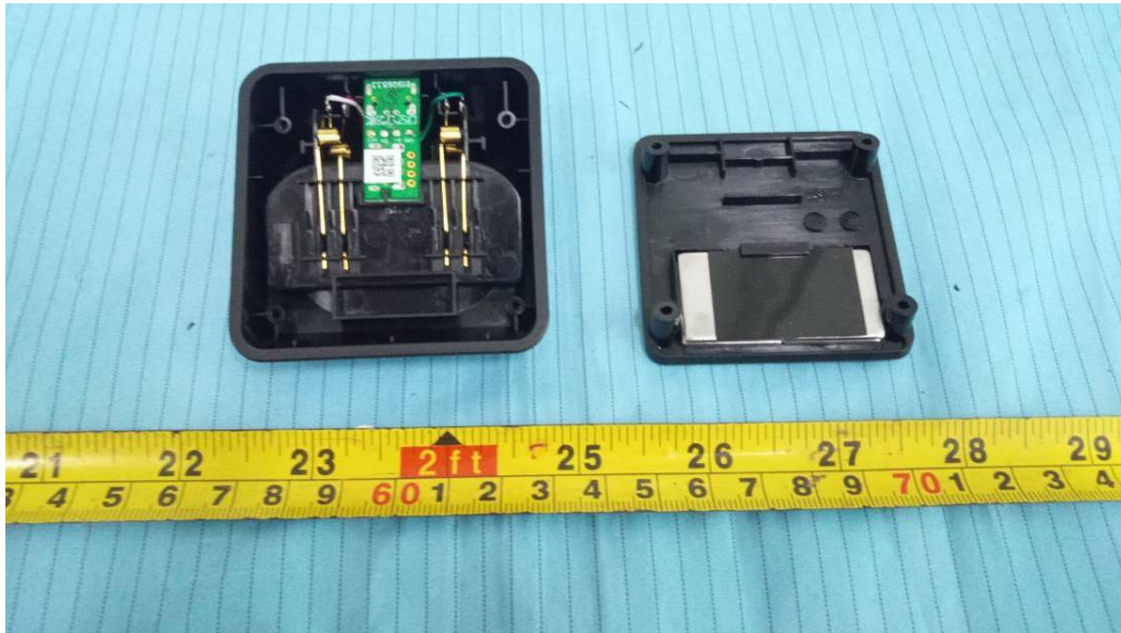
EUT(Charger 2) – Cover off View 1
