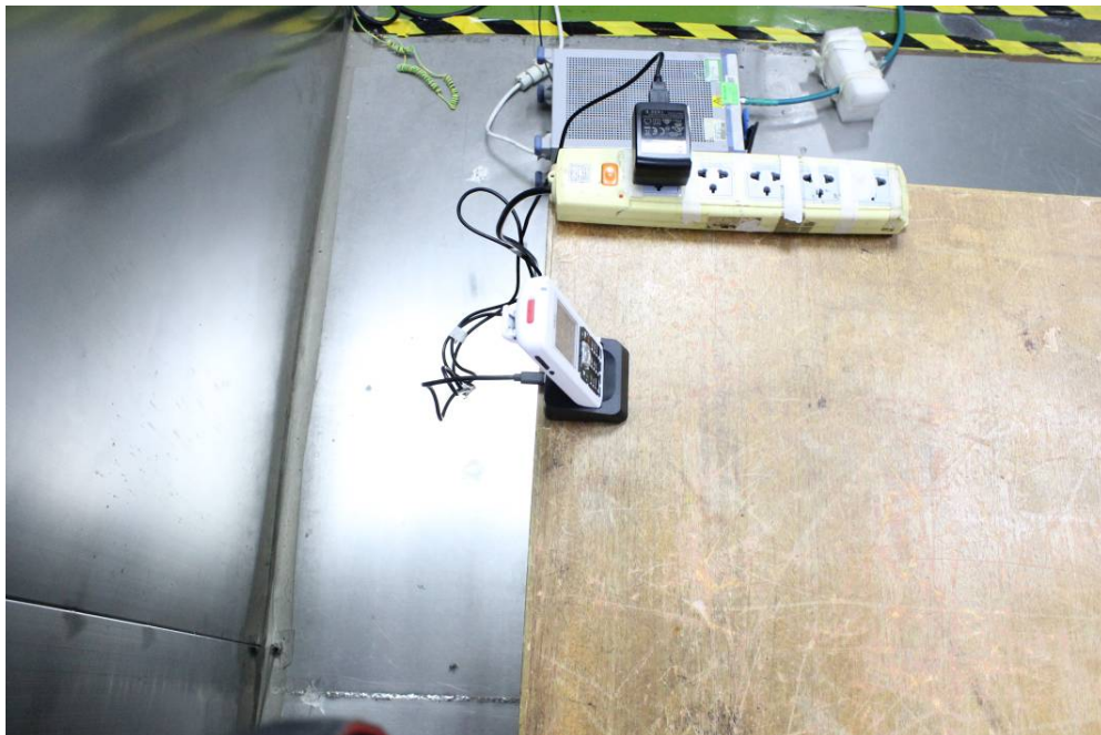
Conducted Emissions - Side View (Charging by Charger 2)
