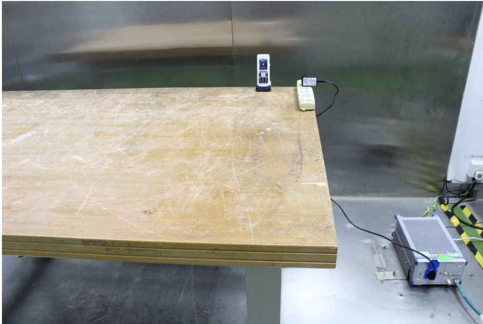
Conducted Emissions - Front View (Charging by Charger 2)
