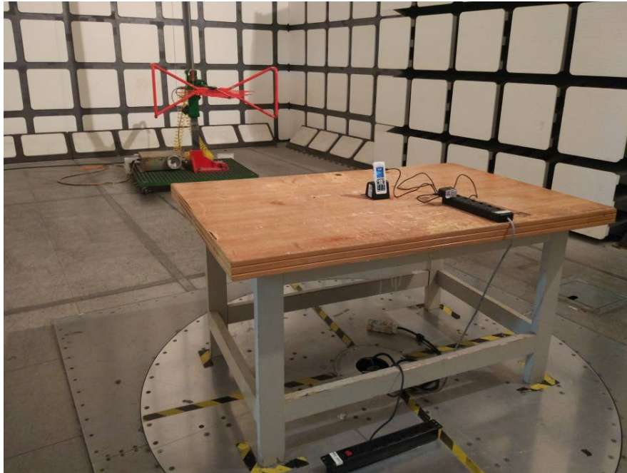
Radiated Emissions View (Below 1 GHz, Charging by Charger 1)
