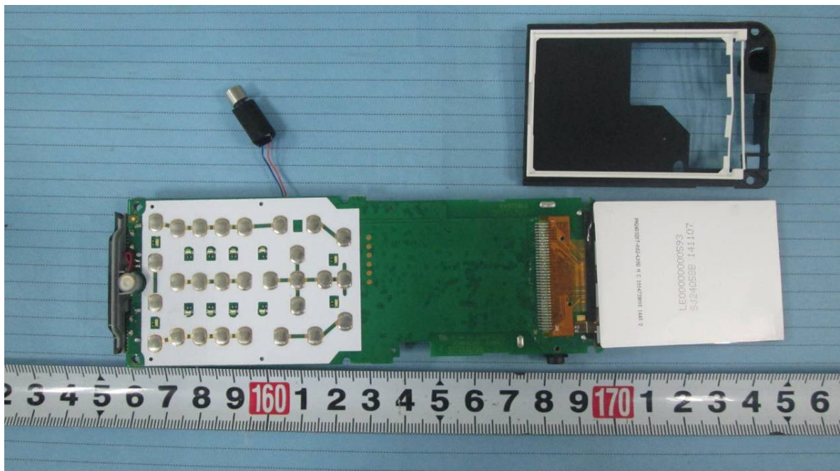
EUT –Main Board Bottom LCD off View
