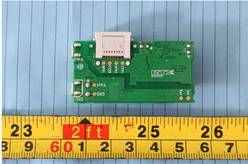
EUT – POE Board Bottom View
