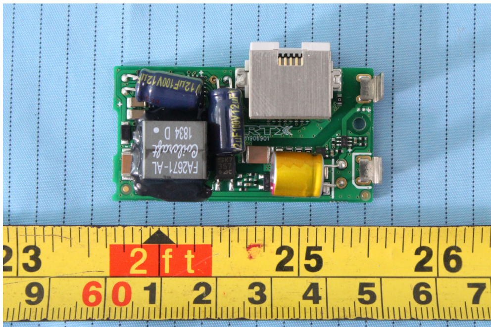
EUT – POE Board Top View
