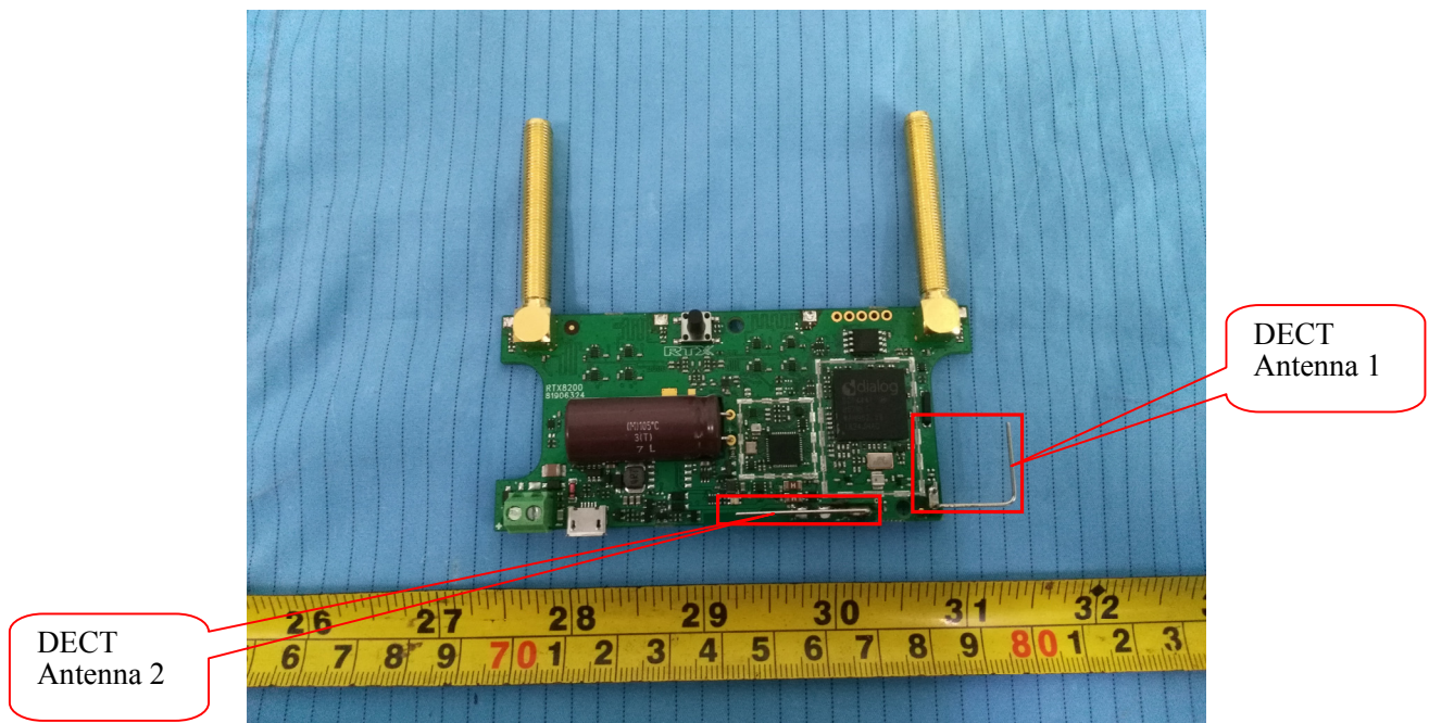
EUT – Main Board Bottom Shielding off View
