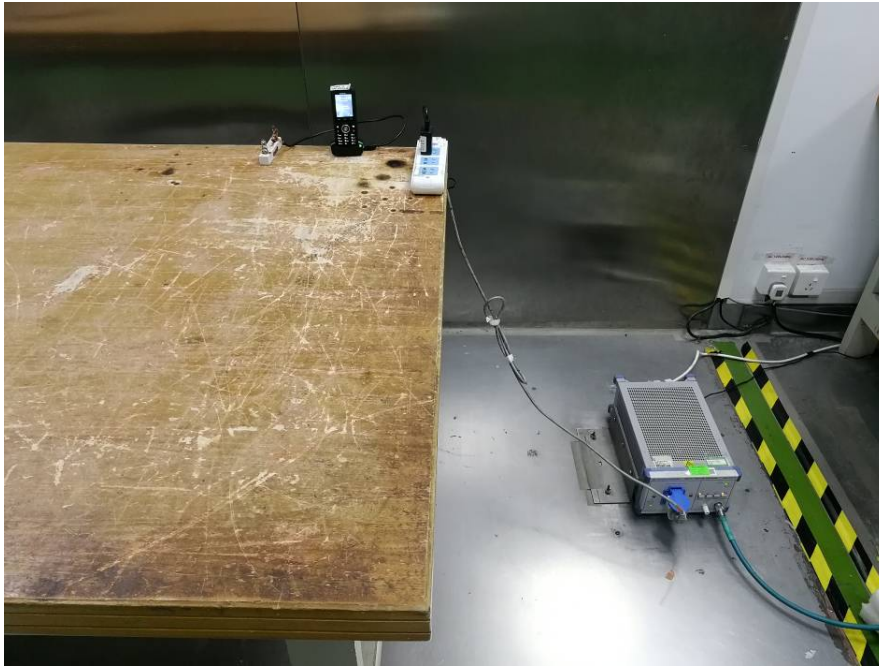
Conducted Emissions - Front View (Adapter 3)
