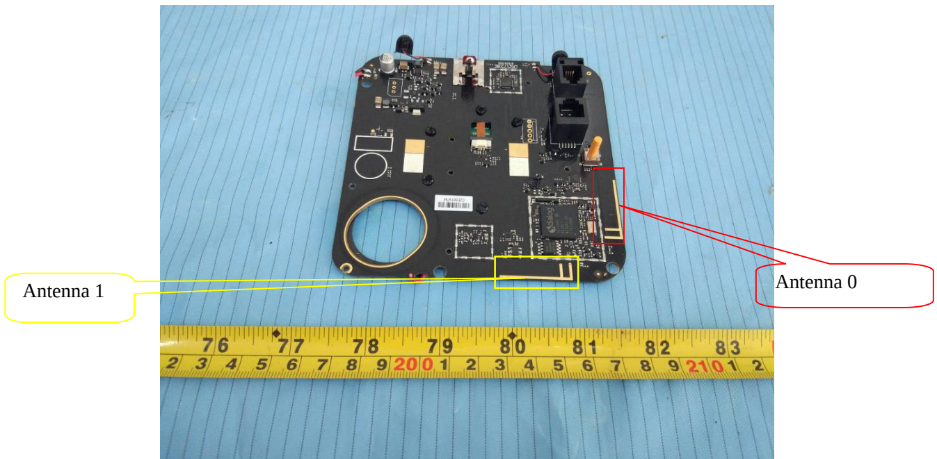
EUT – Main Board Top Shilding off View
