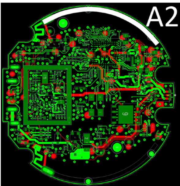
Antenna 2
