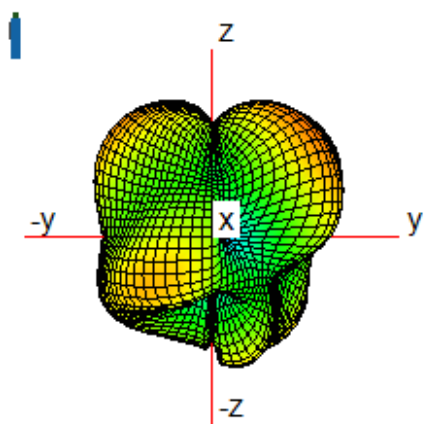
Antenna 2
