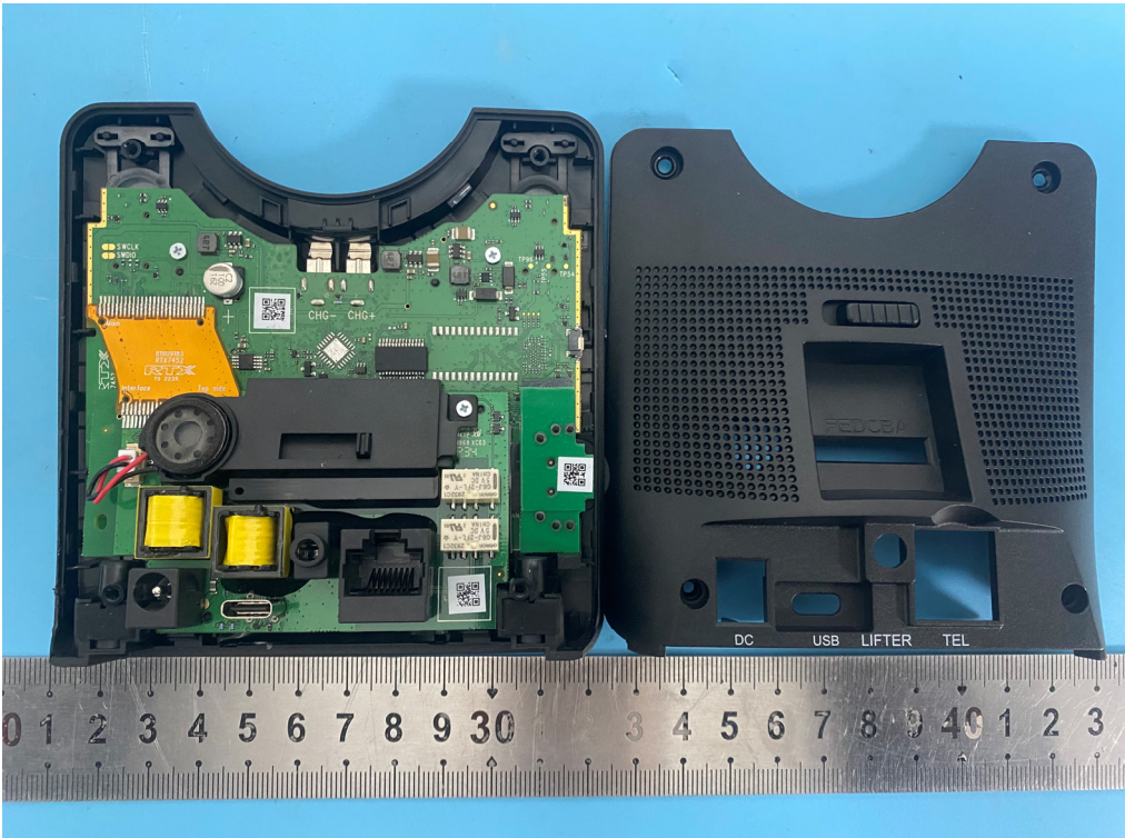
With IC10 (SSOP28)
