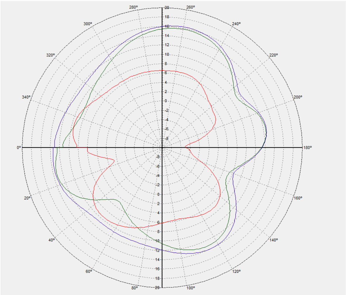
Radiation pattern of DECT antenna A2
