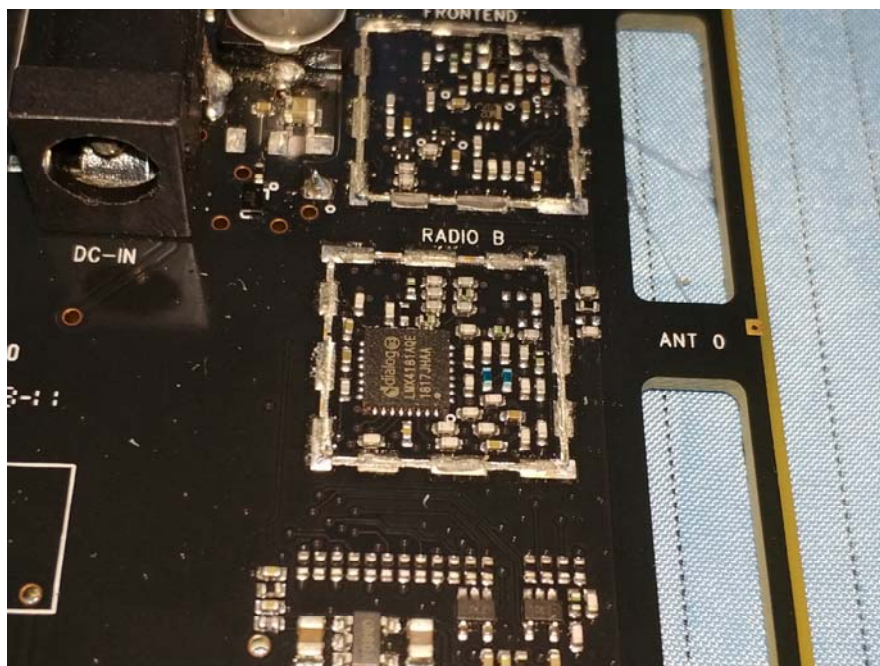
EUT – Radio B View
