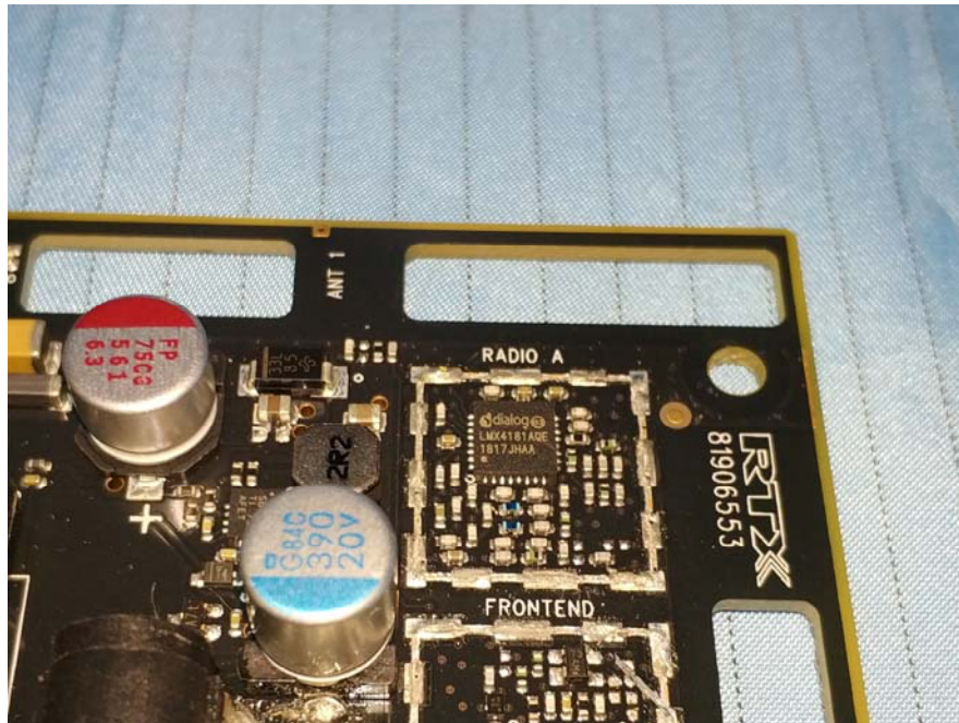
EUT – Radio A View
