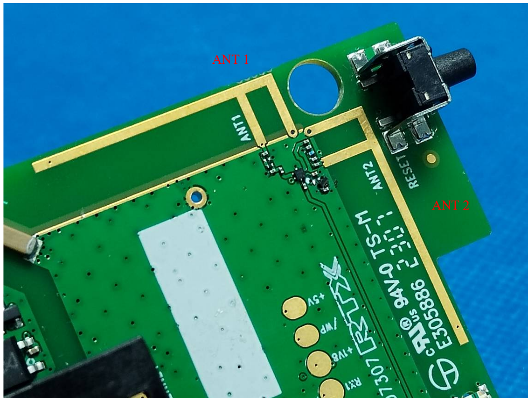
Model: 8328 SIP-DECT SINGLE BASE STATION
