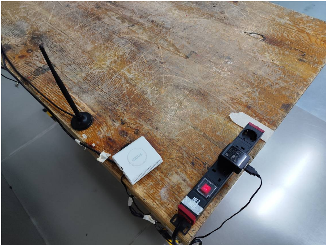
Conducted Emissions Side View-Powered by Adapter 1 (Model RTX9431)
