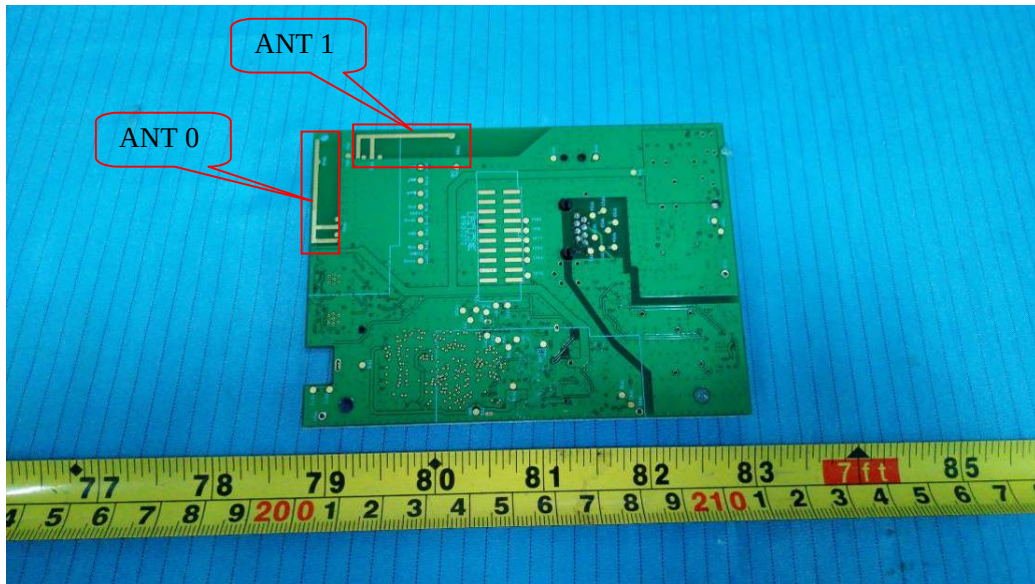
EUT – Main Board Bottom Shielding off View
