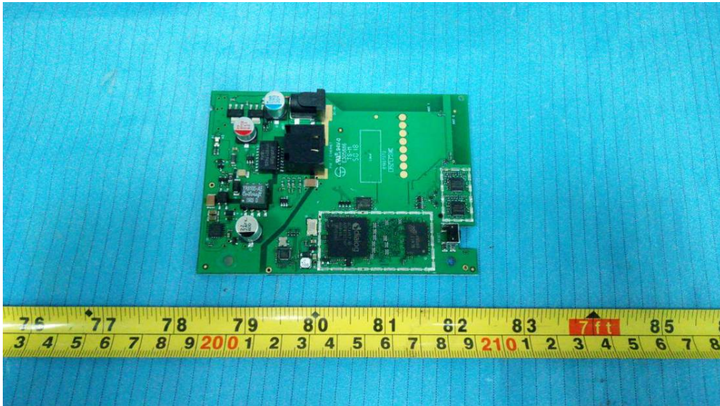
EUT – Main Board Top Shielding off View
