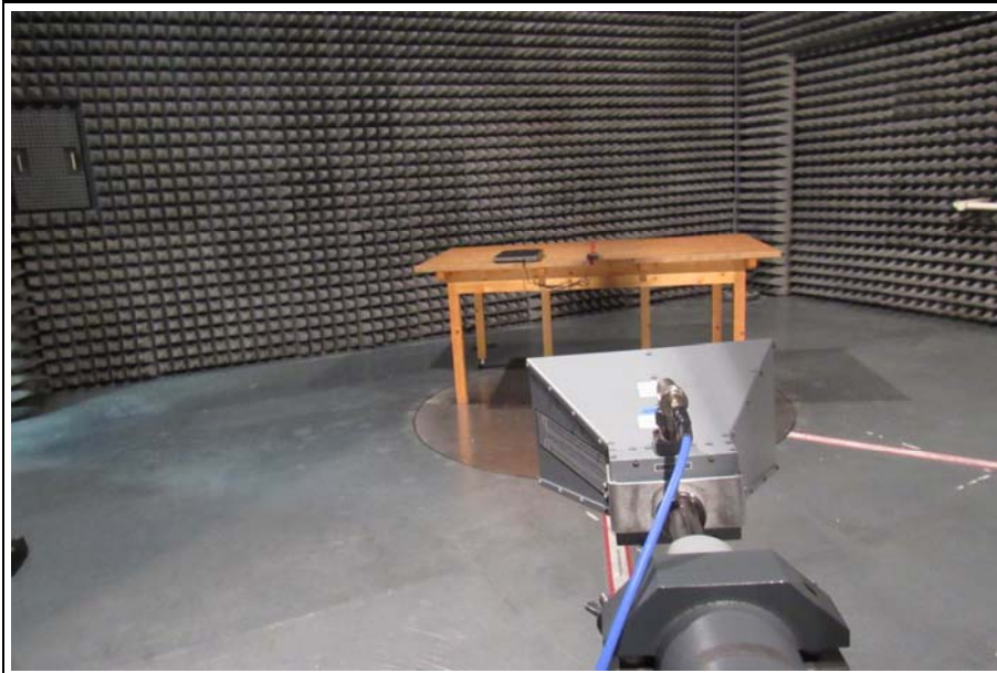
Setup Radiated
