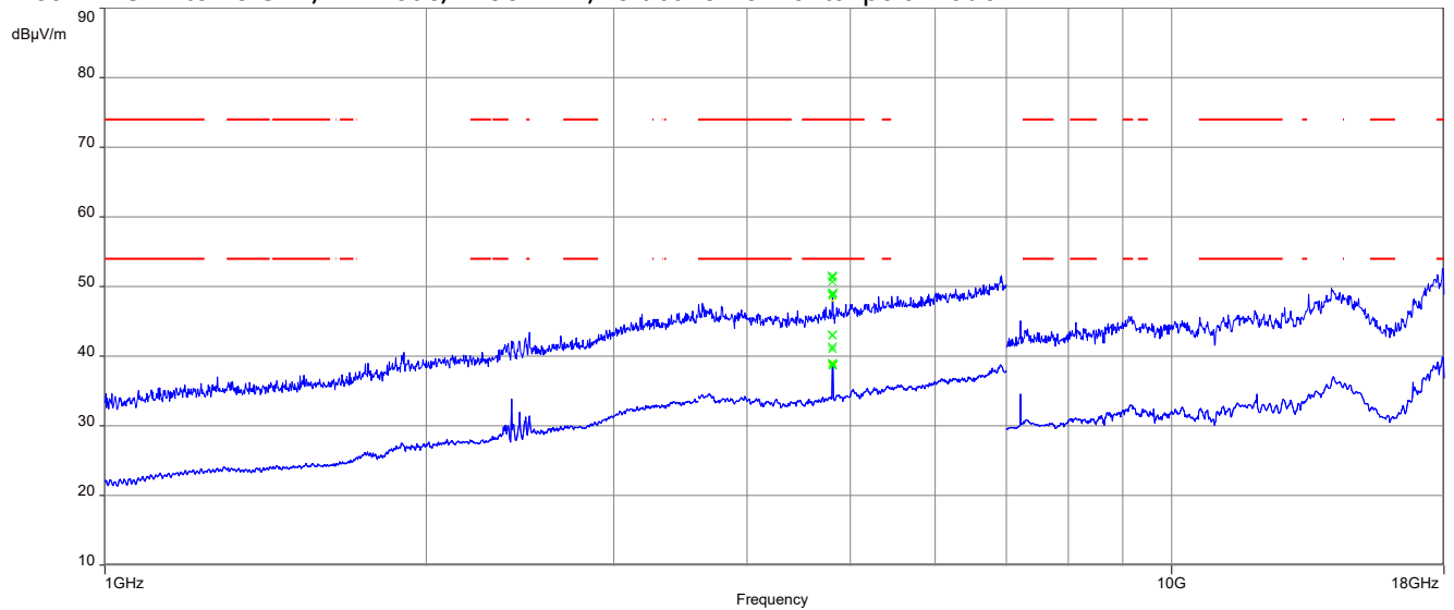
Plot 1: 1 GHz to 18 GHz, TX mode, 2405 MHz, vertical & horizontal polarization
