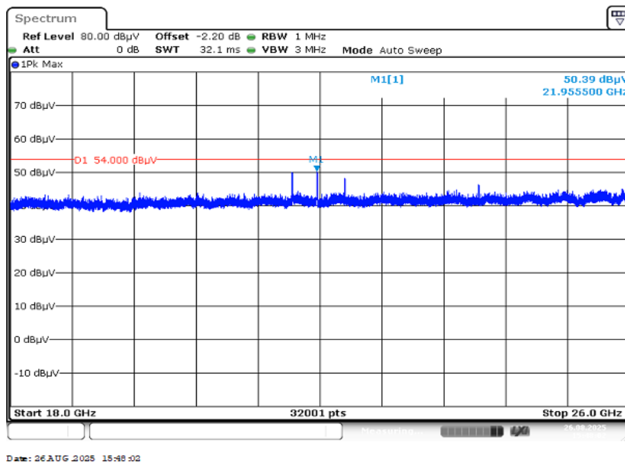
Plot 4: 18 GHz to 26 GHz, TX mode, 2480 MHz, vertical & horizontal polarization
