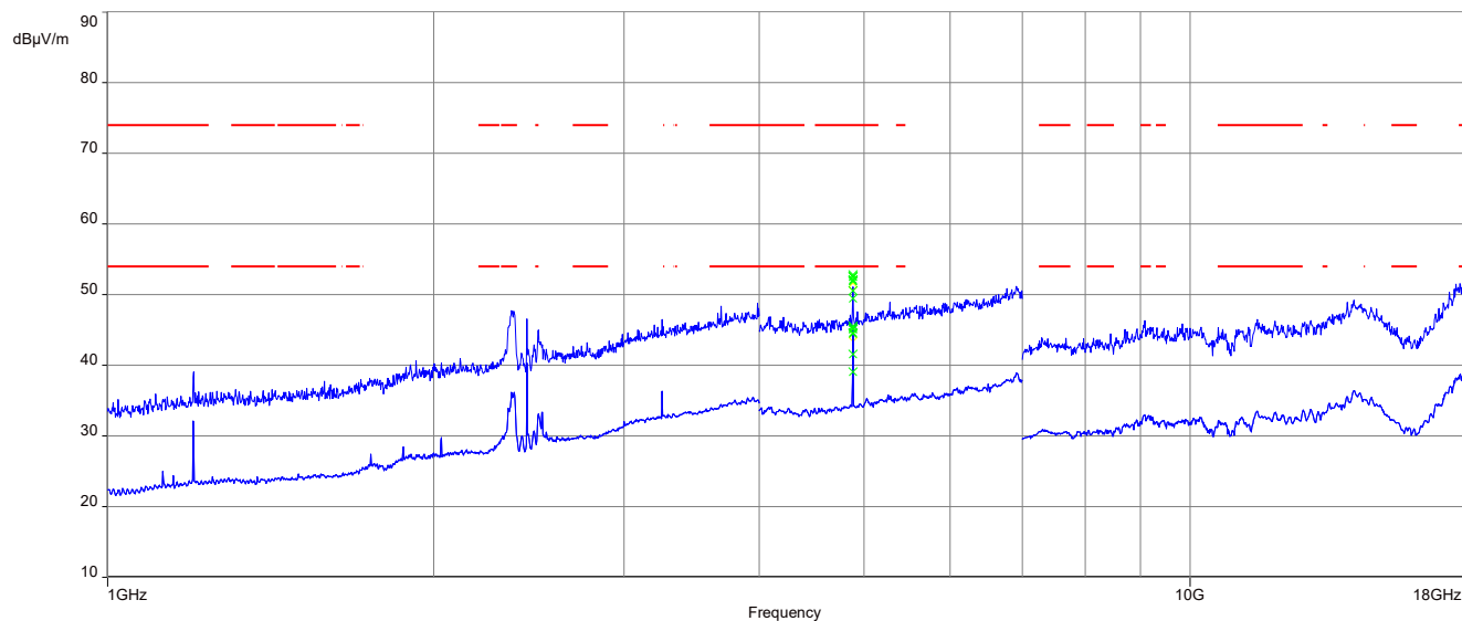
Plot 2: 1 GHz to 18 GHz, TX mode, 2440 MHz, vertical & horizontal polarization, 1 Msps, Taoglas GW.51.5153
