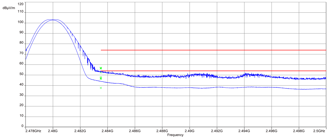
Plot 2: Upper restricted band, 1 Msps, Taoglas GW.51.5153
