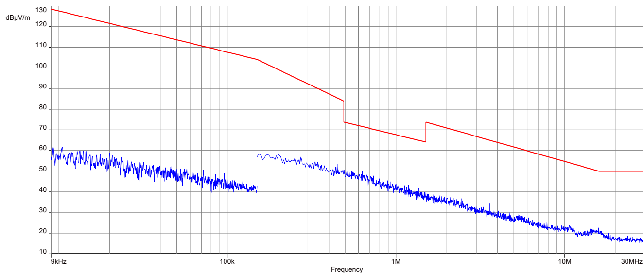
Plot 3: 9 kHz to 30 MHz, 2480 MHz, transmit mode, 1 Msps, Taoglas GW.51.5153
