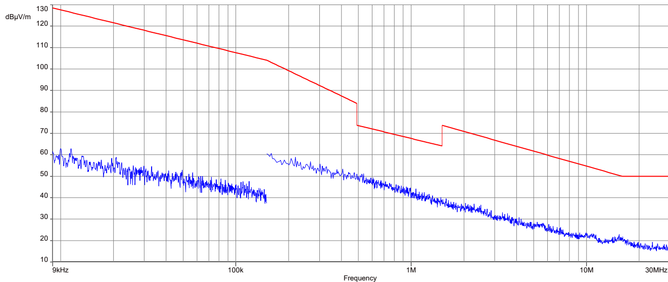
Plot 5: 9 kHz to 30 MHz, 2440 MHz, transmit mode, 2 Msps, Taoglas GW.51.5153
