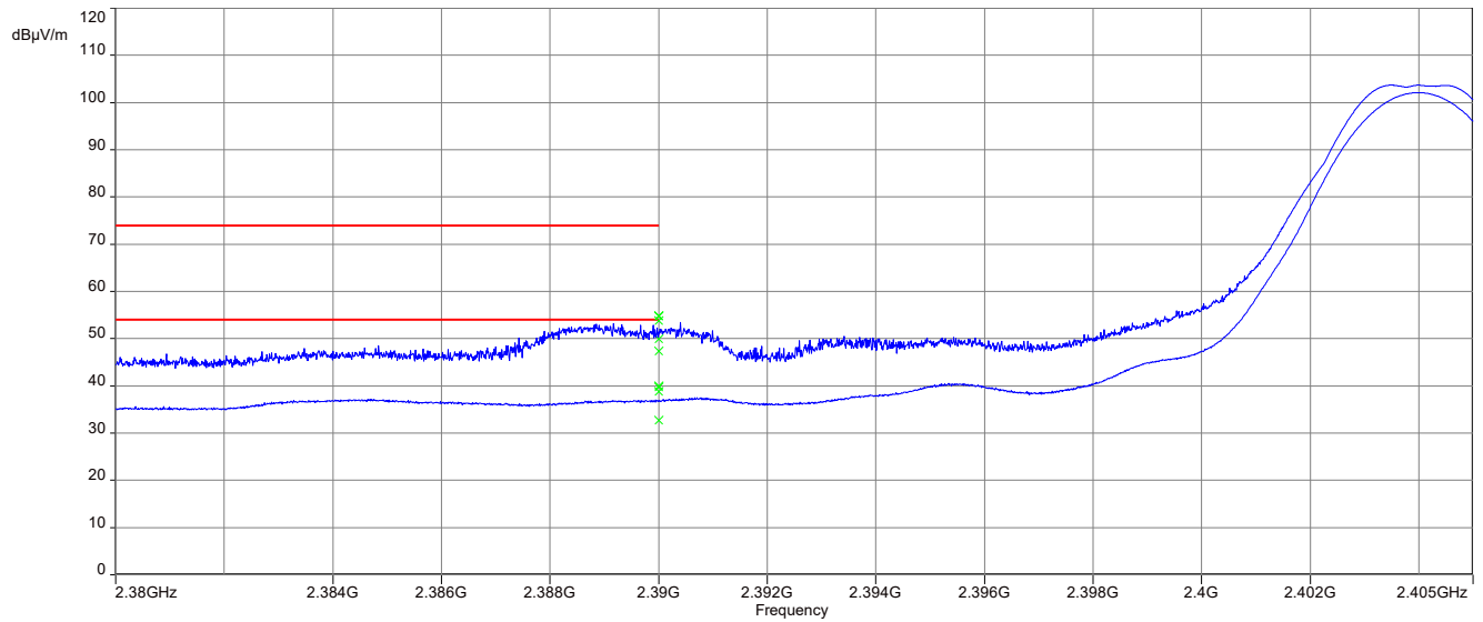
Plot 3: Lower restricted band, 2 Msps, Taoglas GW.51.5153
