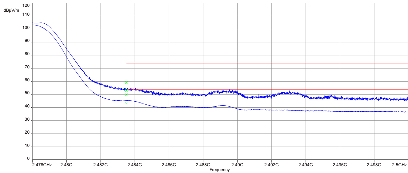
Plot 8: Upper restricted band, 2 Msps, 2J Antennas 2JF1002P
