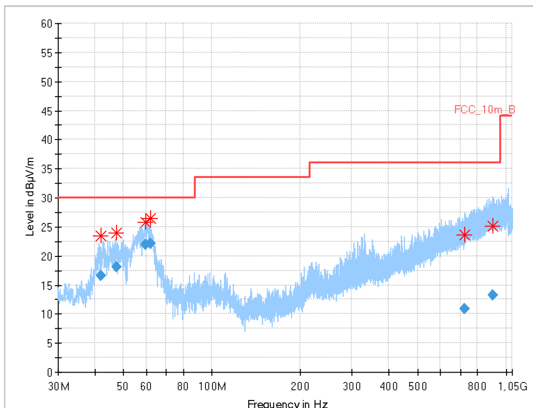
Plot 2: 30 MHz to 1 GHz, TX mode, vertical & horizontal polarization, 2 Msps, valid for all channels, Taoglas GW.51.5153
