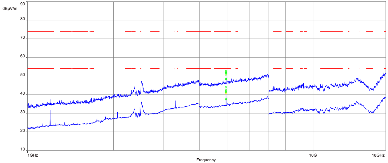
Plot 7: 1 GHz to 18 GHz, TX mode, 2478 MHz, vertical & horizontal polarization, 2 Msps, Taoglas GW.51.5153
