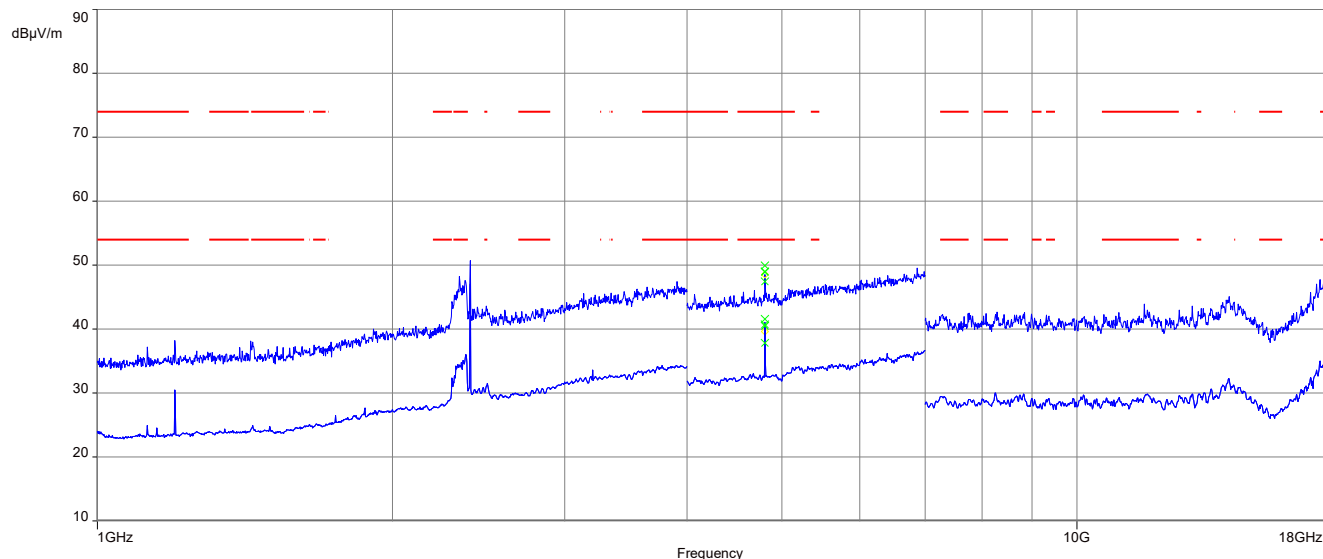
Plot 1: 1 GHz to 18 GHz, TX mode, 2402 MHz, vertical & horizontal polarization, 1 Msps, Taoglas GW.51.5153
