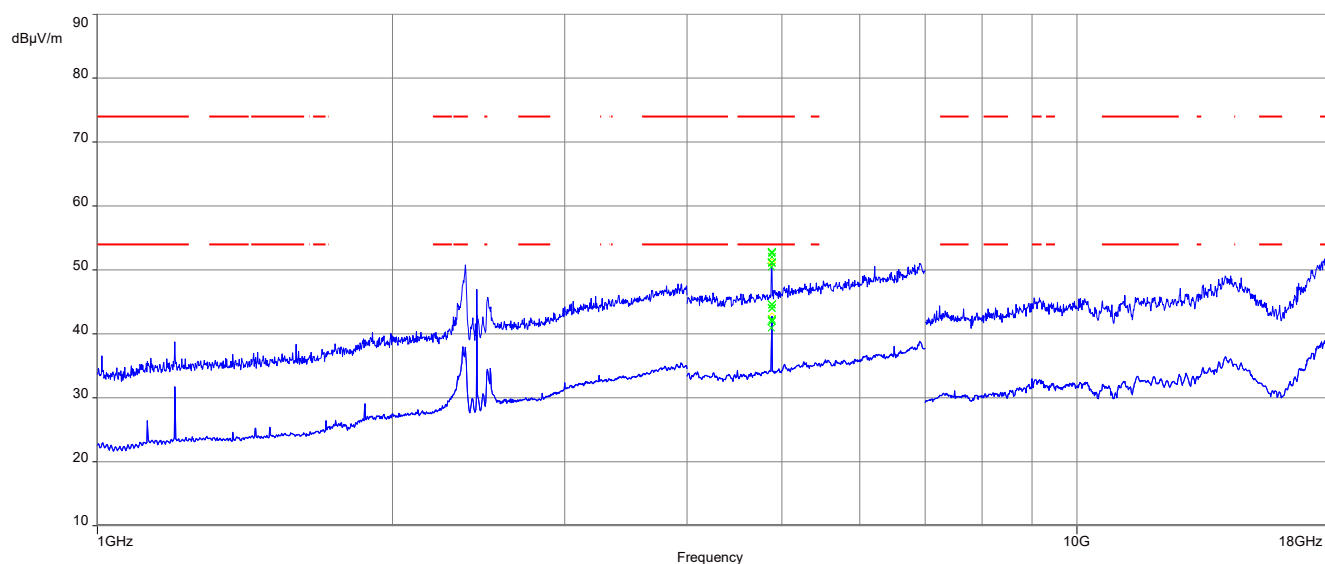
Plot 14: 1 GHz to 18 GHz, TX mode, 2440 MHz, vertical & horizontal polarization, 2 Msps, 2J Antennas 2JF1002P
