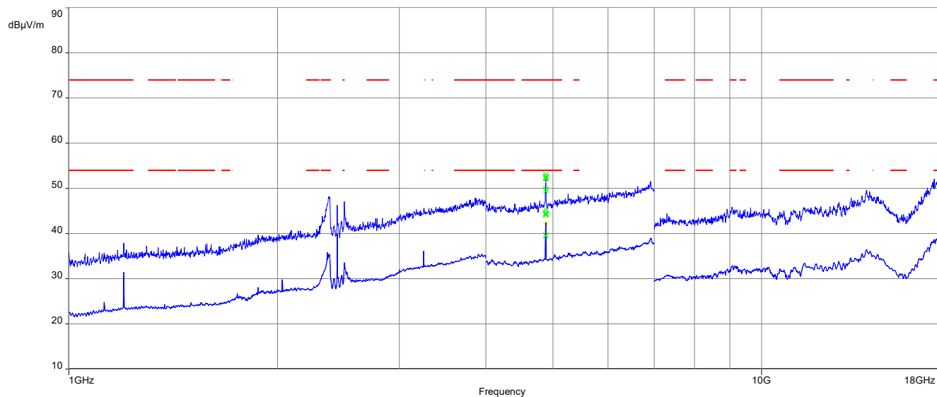
Plot 6: 1 GHz to 18 GHz, TX mode, 2440 MHz, vertical & horizontal polarization, 2 Msps, Taoglas GW.51.5153
