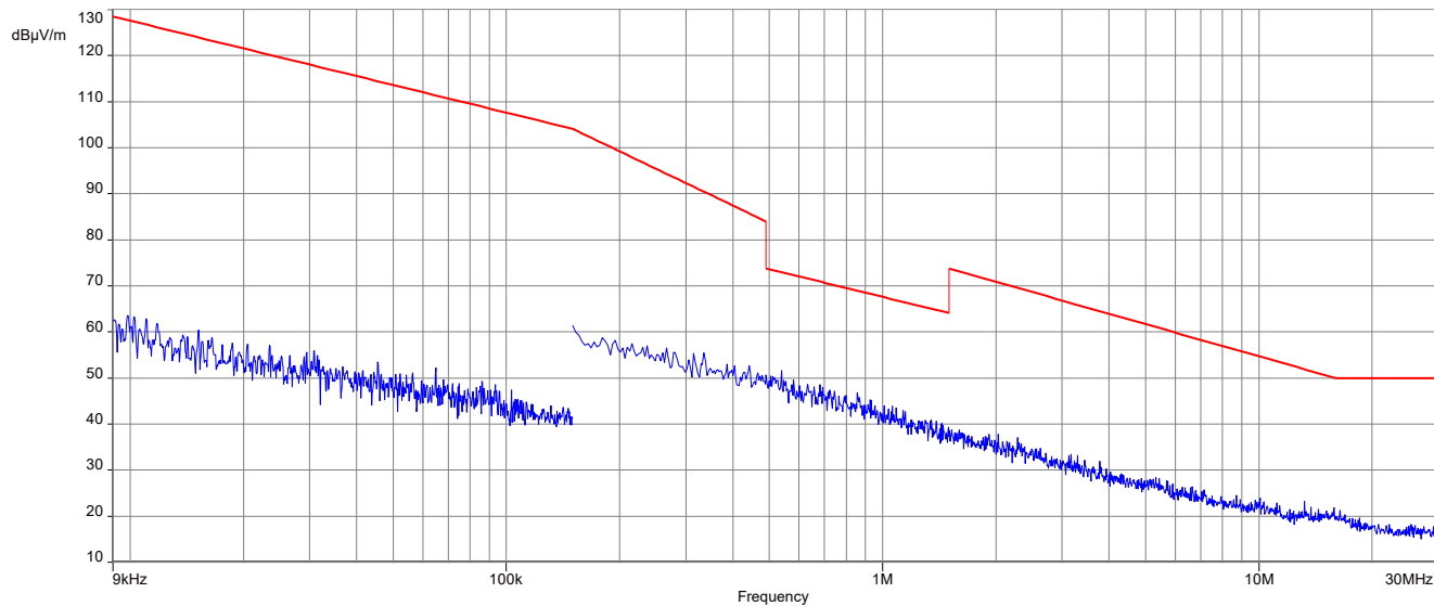
Plot 10: 9 kHz to 30 MHz, 2404 MHz, transmit mode, 2 Msps, 2J Antennas 2JF1002P
