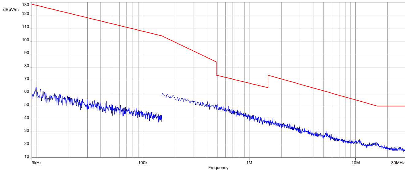
Plot 1: 9 kHz to 30 MHz, 2402 MHz, transmit mode, 1 Msps, Taoglas GW.51.5153
