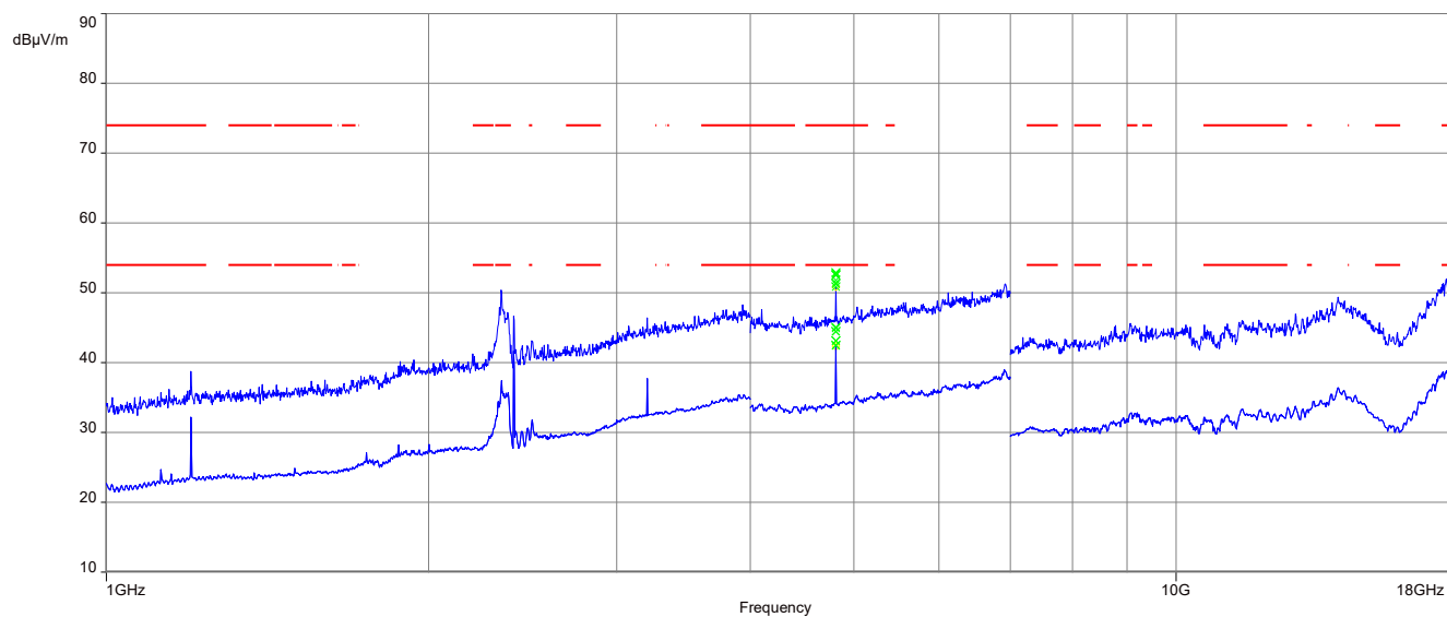
Plot 5: 1 GHz to 18 GHz, TX mode, 2404 MHz, vertical & horizontal polarization, 2 Msps, Taoglas GW.51.5153
