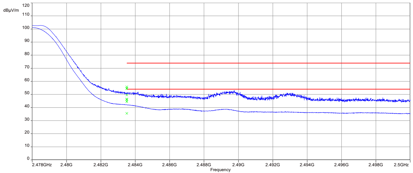
Plot 4: Upper restricted band, 2 Msps, Taoglas GW.51.5153
