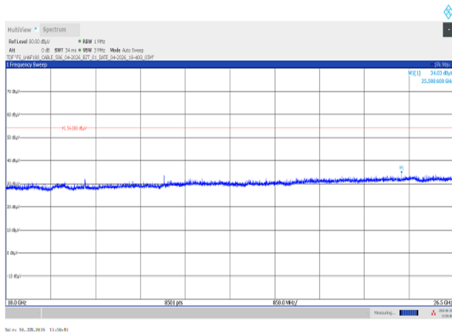
Plot 8: 18 GHz to 26 GHz, TX mode, 2478 MHz, vertical & horizontal polarization, 2 Msps, Taoglas GW.51.5153
