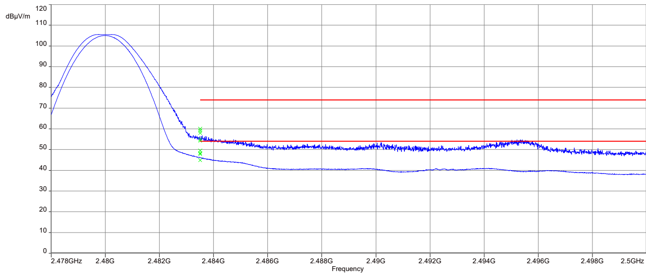
Plot 6: Upper restricted band, 1 Msps, 2J Antennas 2JF1002P
