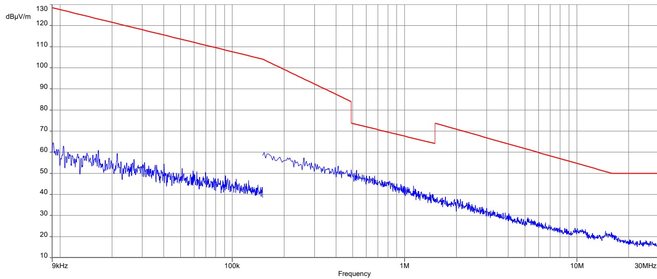
Plot 4: 9 kHz to 30 MHz, 2404 MHz, transmit mode, 2 Msps, Taoglas GW.51.5153
