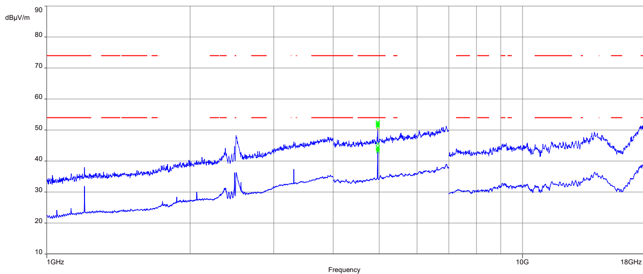
Plot 3: 1 GHz to 18 GHz, TX mode, 2480 MHz, vertical & horizontal polarization, 1 Msps, Taoglas GW.51.5153
