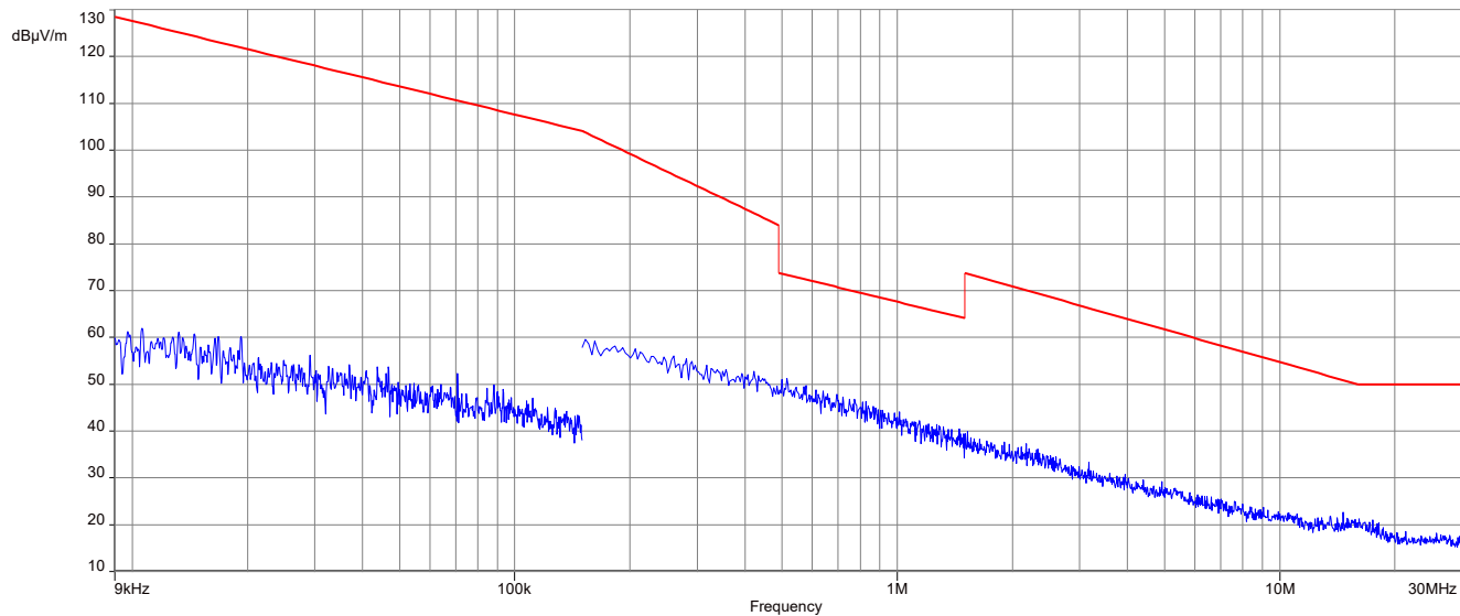
Plot 8: 9 kHz to 30 MHz, 2440 MHz, transmit mode, 1 Msps, 2J Antennas 2JF1002P
