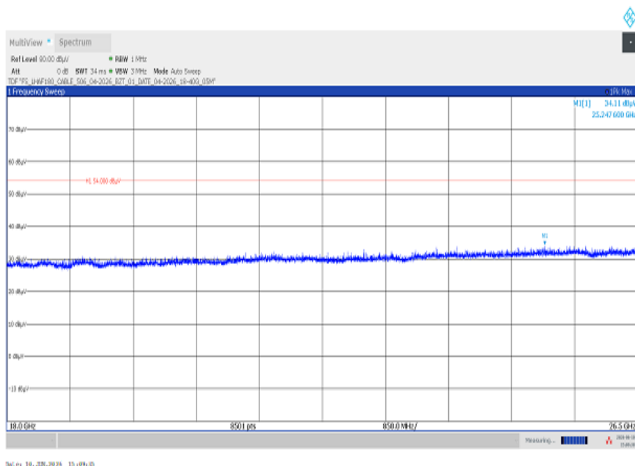
Plot 12: 18 GHz to 26 GHz, TX mode, 2480 MHz, vertical & horizontal polarization, 1 Msps, 2J Antennas 2JF1002P
