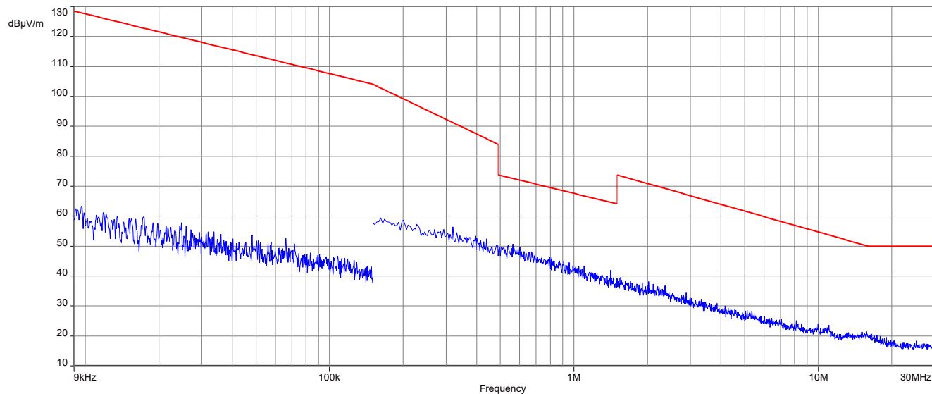
Plot 11: 9 kHz to 30 MHz, 2440 MHz, transmit mode, 2 Msps, 2J Antennas 2JF1002P
