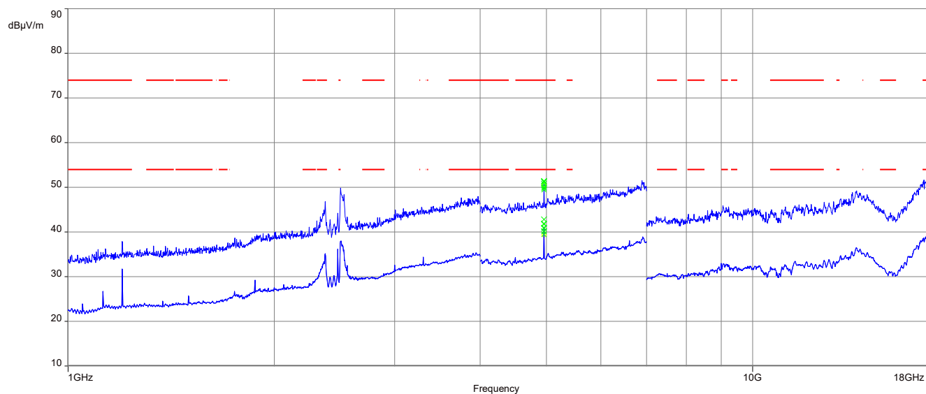
Plot 15: 1 GHz to 18 GHz, TX mode, 2478 MHz, vertical & horizontal polarization, 2 Msps, 2J Antennas 2JF1002P
