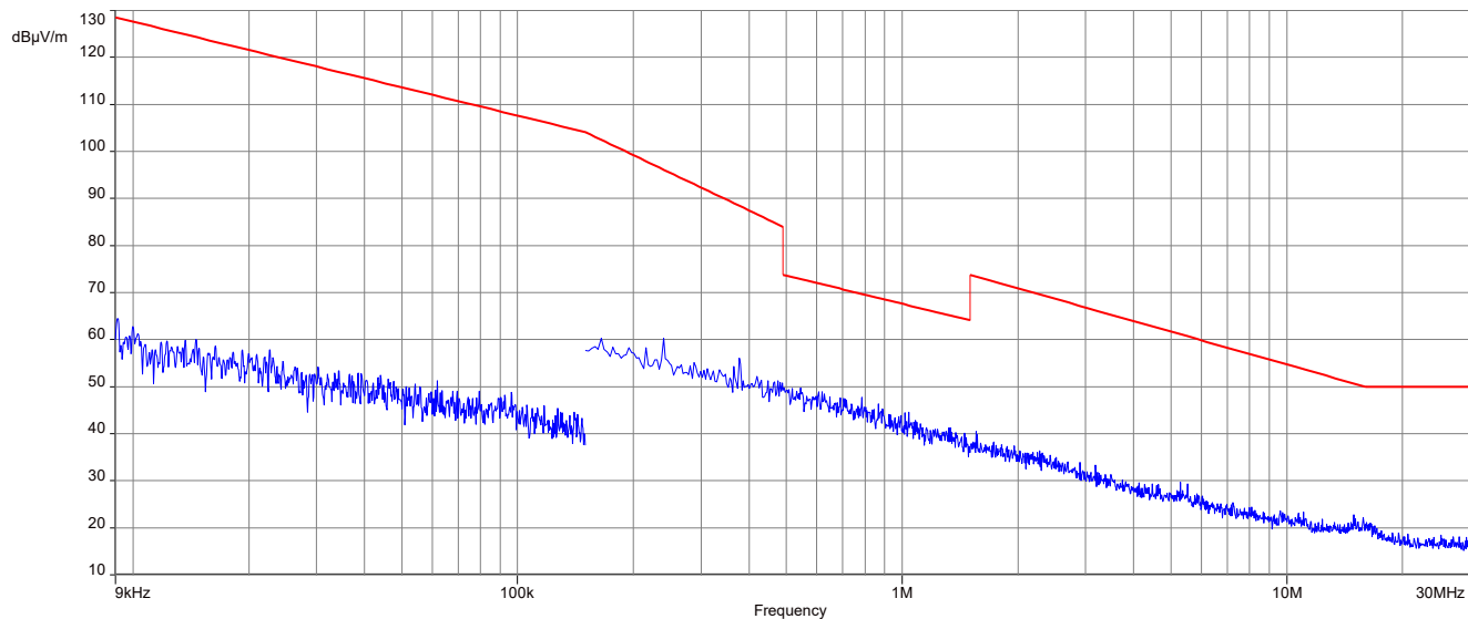
Plot 7: 9 kHz to 30 MHz, 2402 MHz, transmit mode, 1 Msps, 2J Antennas 2JF1002P
