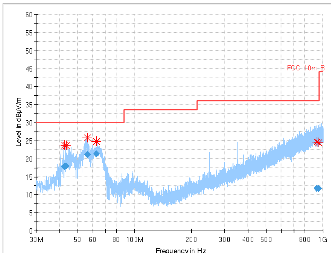
Plot 4: 30 MHz to 1 GHz, TX mode, vertical & horizontal polarization, 2 Msps, valid for all channels, 2J Antennas 2JF1002P
