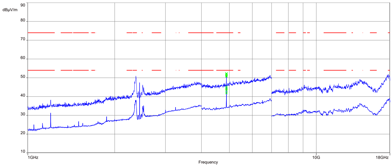
Plot 10: 1 GHz to 18 GHz, TX mode, 2440 MHz, vertical & horizontal polarization, 1 Msps, 2J Antennas 2JF1002P
