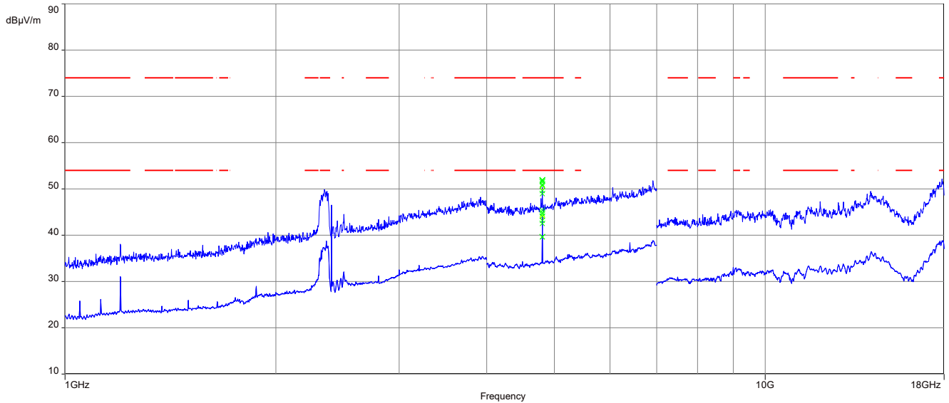
Plot 9: 1 GHz to 18 GHz, TX mode, 2402 MHz, vertical & horizontal polarization, 1 Msps, 2J Antennas 2JF1002P
