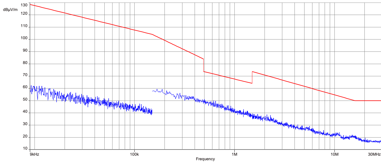
Plot 2: 9 kHz to 30 MHz, 2440 MHz, transmit mode, 1 Msps, Taoglas GW.51.5153
