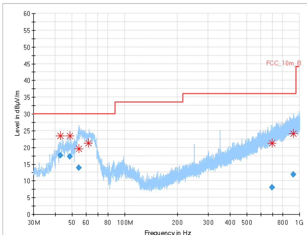
Plot 3: 30 MHz to 1 GHz, TX mode, vertical & horizontal polarization, 1 Msps, valid for all channels, 2J Antennas 2JF1002P
