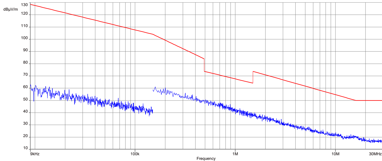
Plot 12: 9 kHz to 30 MHz, 2478 MHz, transmit mode, 2 Msps, 2J Antennas 2JF1002P
