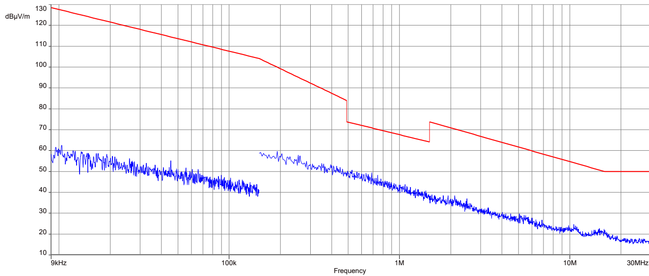
Plot 6: 9 kHz to 30 MHz, 2478 MHz, transmit mode, 2 Msps, Taoglas GW.51.5153
