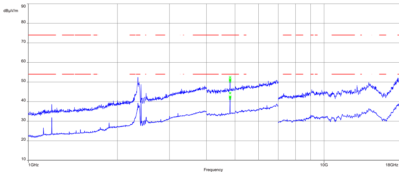
Plot 13: 1 GHz to 18 GHz, TX mode, 2404 MHz, vertical & horizontal polarization, 2 Msps, 2J Antennas 2JF1002P
