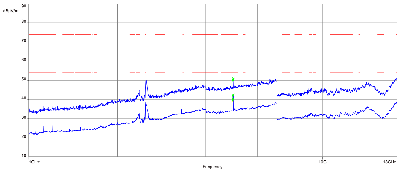
Plot 11: 1 GHz to 18 GHz, TX mode, 2480 MHz, vertical & horizontal polarization, 1 Msps, 2J Antennas 2JF1002P
