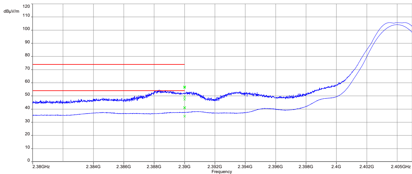
Plot 7: Lower restricted band, 2 Msps, 2J Antennas 2JF1002P
