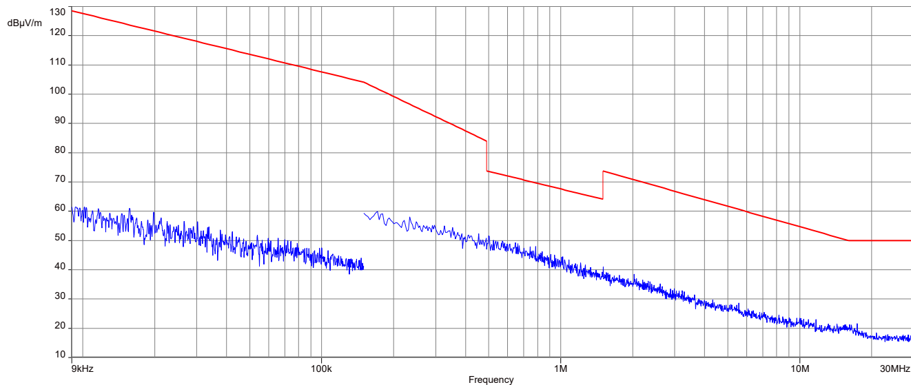
Plot 9: 9 kHz to 30 MHz, 2480 MHz, transmit mode, 1 Msps, 2J Antennas 2JF1002P
