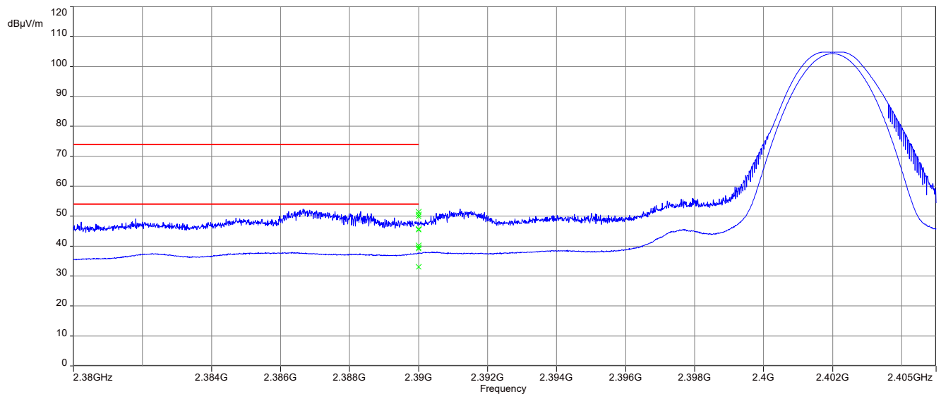
Plot 1: Lower restricted band, 1 Msps, Taoglas GW.51.5153
