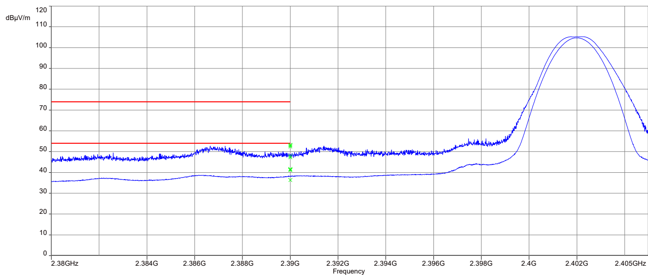
Plot 5: Lower restricted band, 1 Msps, 2J Antennas 2JF1002P
