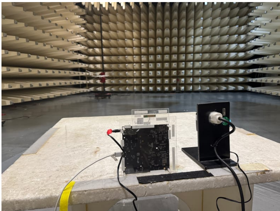
Photo 5: RSE set-up < 1 GHz with 2J antenna
