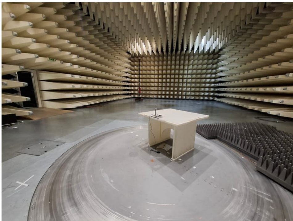
Photo 1: RSE set-up < 1 GHz with Taoglas antenna
