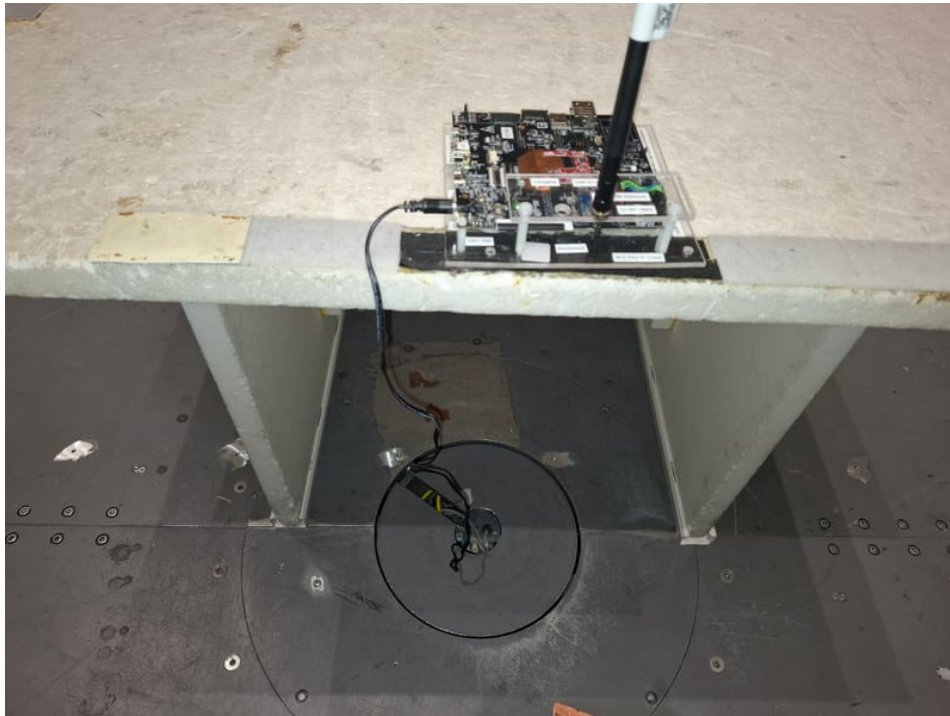
Photo 3: RSE set-up < 1 GHz with Taoglas antenna
