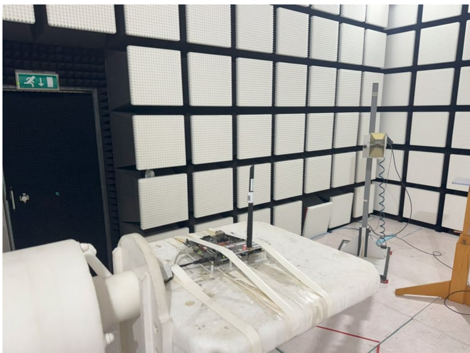
Photo 6: RSE set-up > 1 GHz with Taoglas antenna
