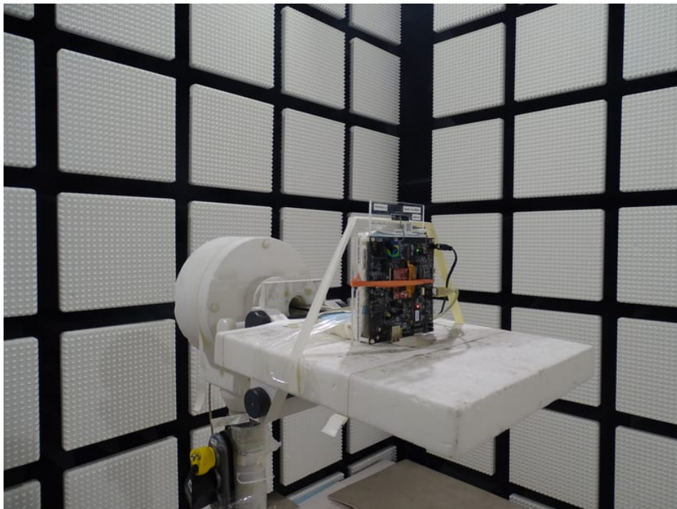
Photo 9: RSE set-up > 1 GHz with 2J antenna
