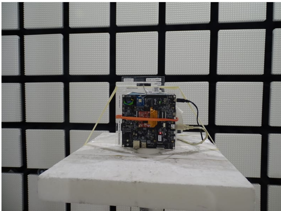
Photo 10: RSE set-up > 1 GHz with 2J antenna
