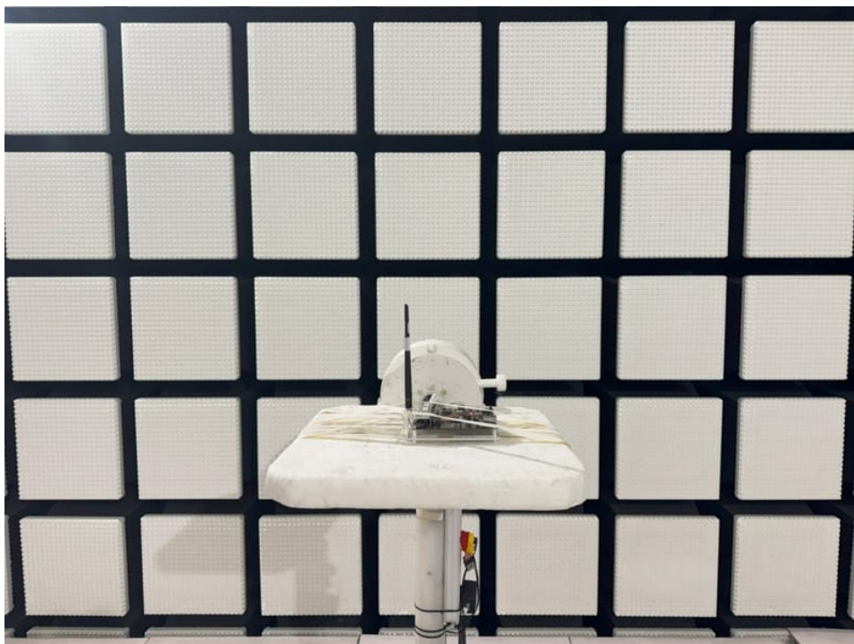
Photo 8: RSE set-up > 1 GHz with Taoglas antenna
