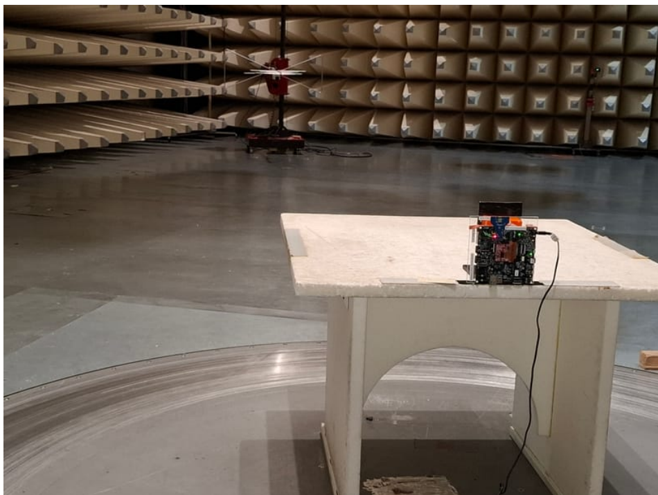
Photo 2: RSE set-up < 1 GHz with chip antenna
