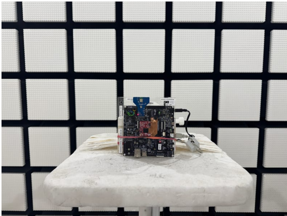
Photo 5: RSE set-up > 1 GHz with chip antenna
