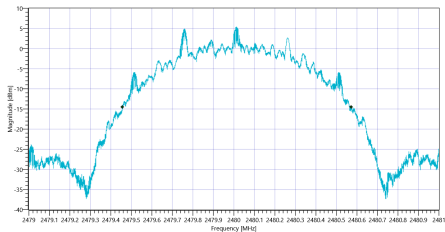
Plot_FCC Part 15.247 Bandwidth 99PCT-20dB ~ BT LE coded S2_16032020_151144.png
