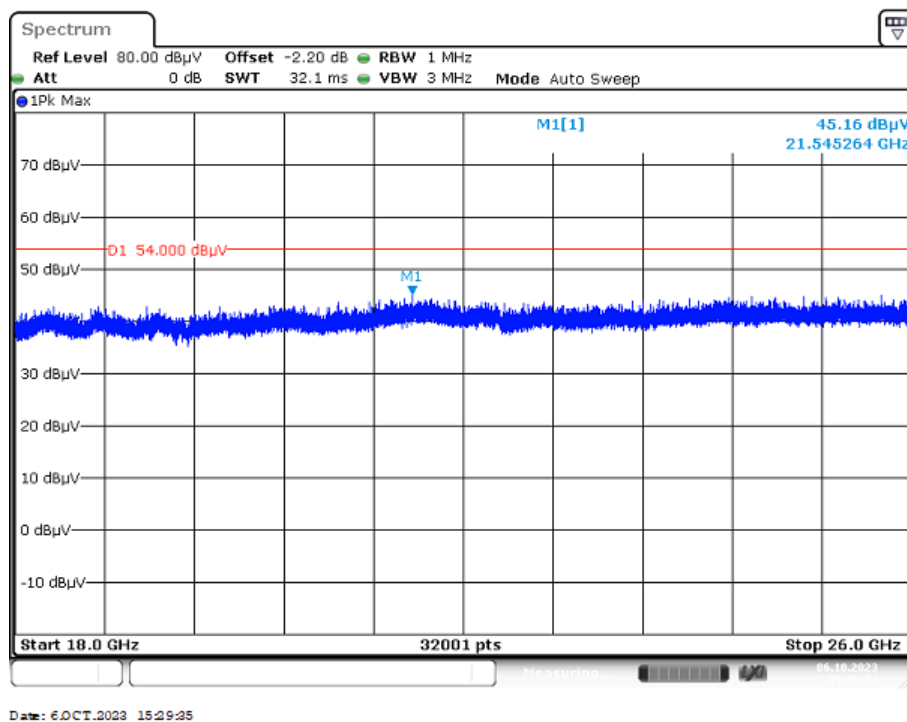
Plot 8: 18 GHz to 26 GHz, TX mode, vertical & horizontal polarization, valid for all channels (external antenna setup)
