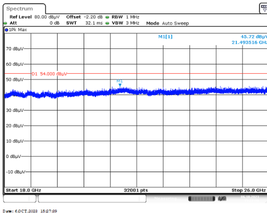
Plot 4: 18 GHz to 26 GHz, TX mode, vertical & horizontal polarization, valid for all channels (internal antenna setup)
