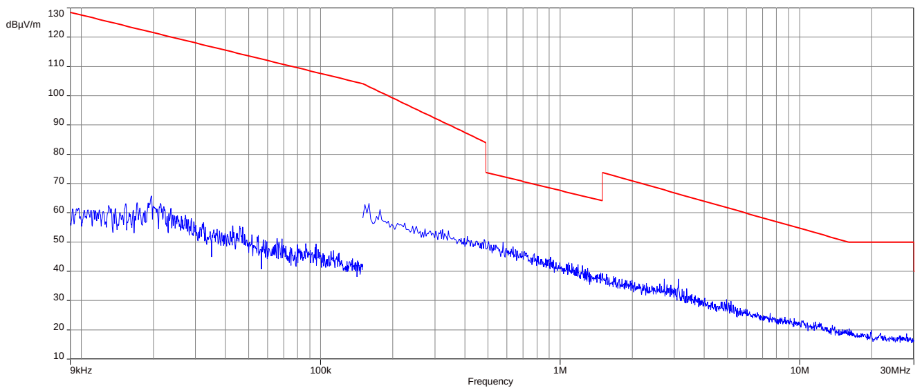
Plot 2: 9 kHz to 30 MHz, 2440 MHz, transmit mode (internal antenna setup)
