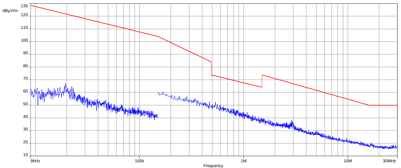
Plot 4: 9 kHz to 30 MHz, 2405 MHz, transmit mode (external antenna setup)
