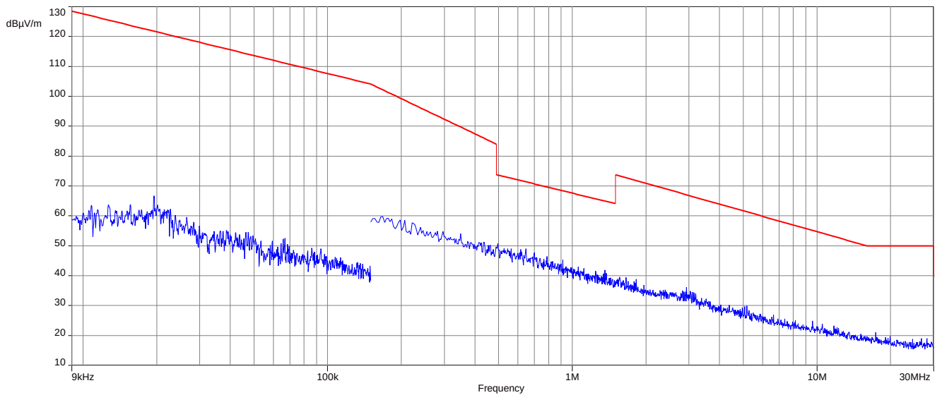
Plot 3: 9 kHz to 30 MHz, 2480 MHz, transmit mode (internal antenna setup)
