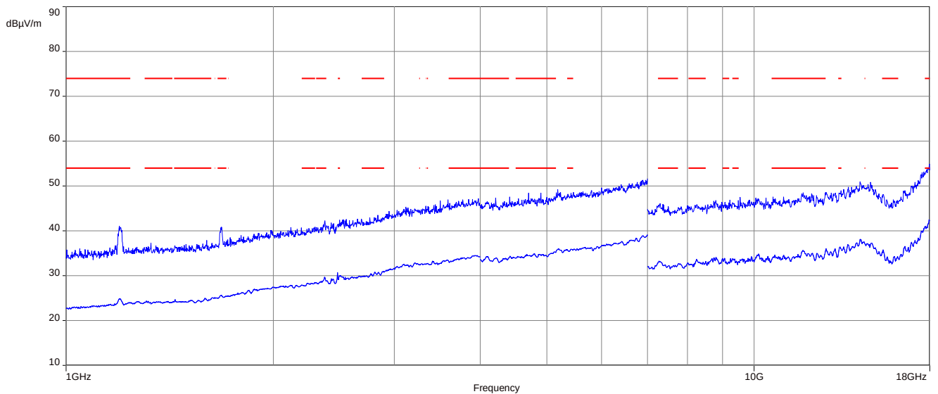
Plot 3: 1 GHz to 18 GHz, TX mode, 2480 MHz, vertical & horizontal polarization (internal antenna setup)
