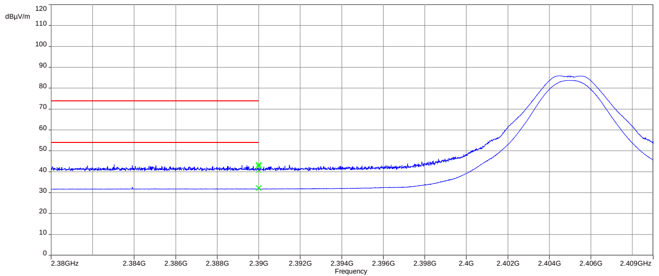
Plot 1: Lower restricted band, 2405 MHz (internal antenna setup)
