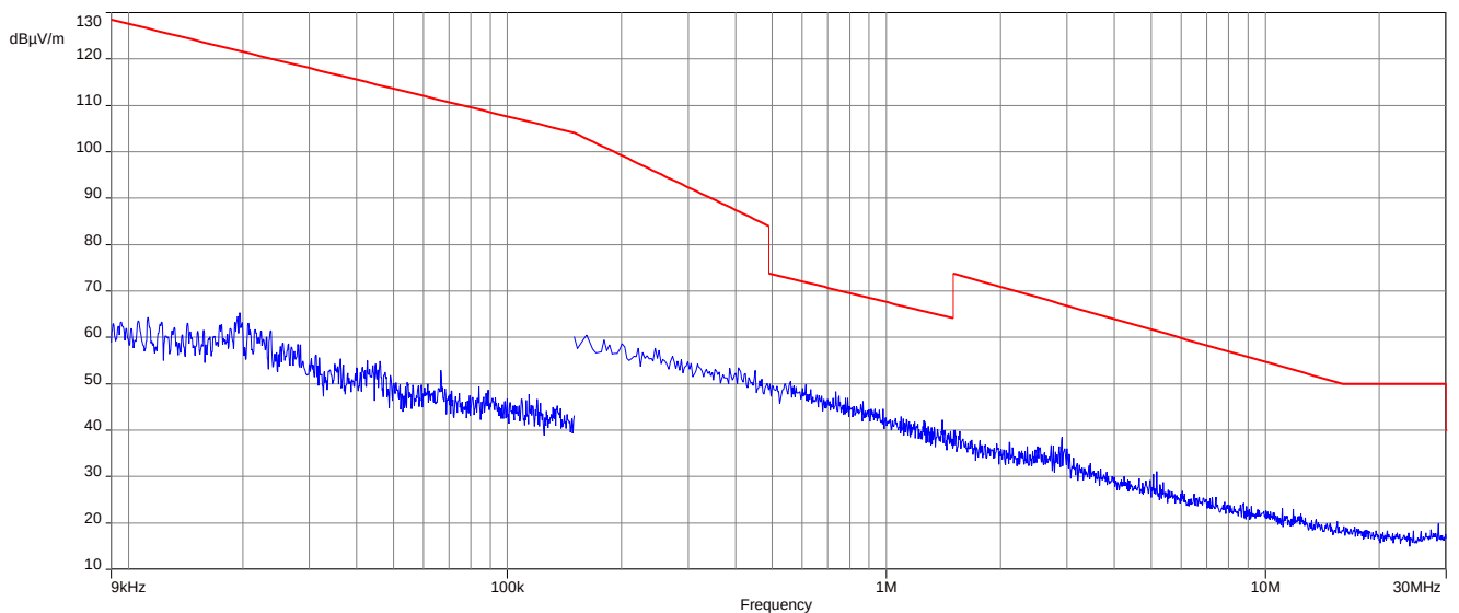
Plot 6: 9 kHz to 30 MHz, 2480 MHz, transmit mode (external antenna setup)
