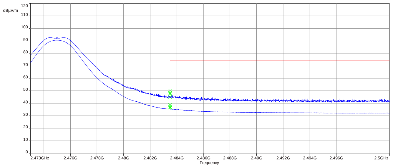
Plot 2: Upper restricted band 2475 MHz (internal antenna setup)
