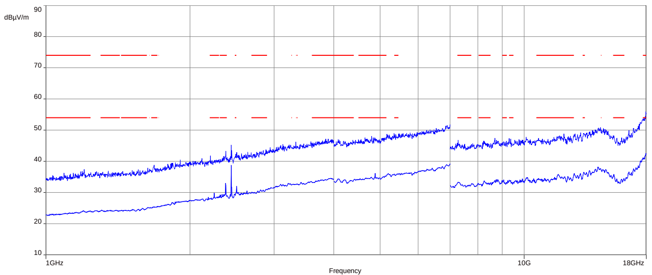
Plot 6: 1 GHz to 18 GHz, TX mode, 2440 MHz, vertical & horizontal polarization (external antenna setup)
