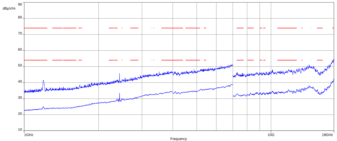
Plot 1: 1 GHz to 18 GHz, TX mode, 2405 MHz, vertical & horizontal polarization (internal antenna setup)
