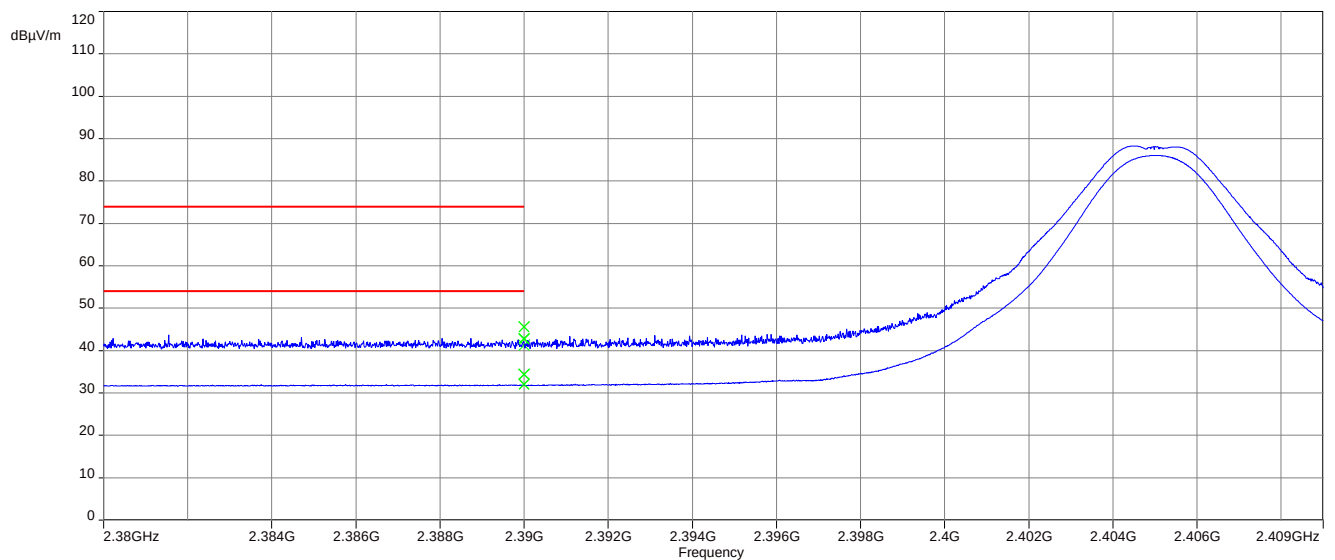
Plot 4: Lower restricted band, 2405 MHz (external antenna setup)
