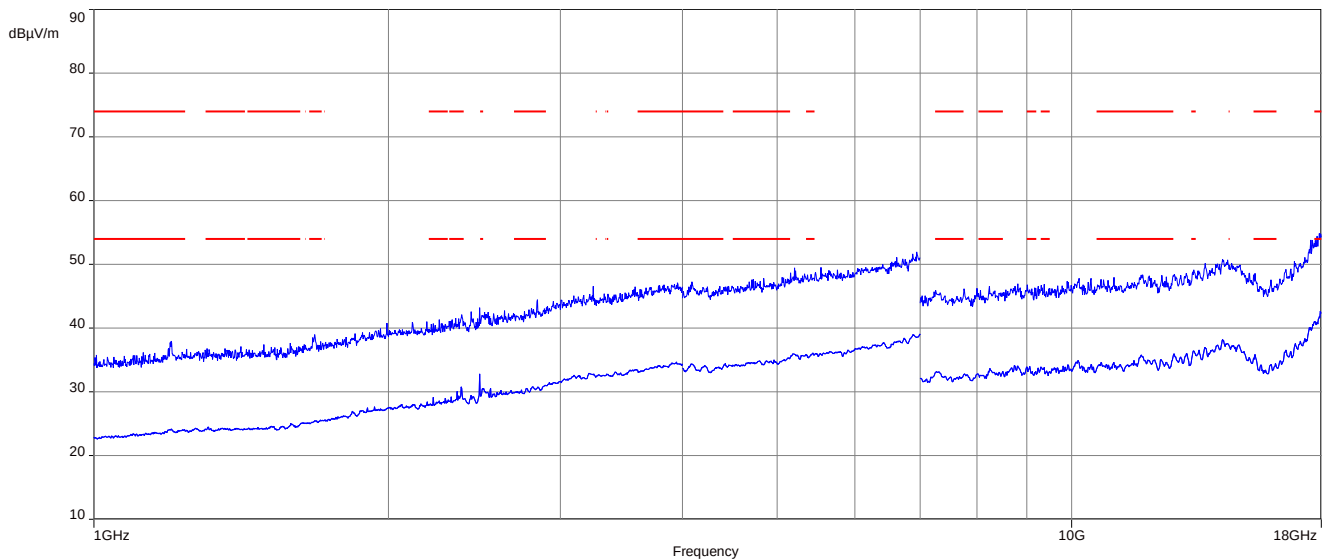
Plot 7: 1 GHz to 18 GHz, TX mode, 2480 MHz, vertical & horizontal polarization (external antenna setup)
