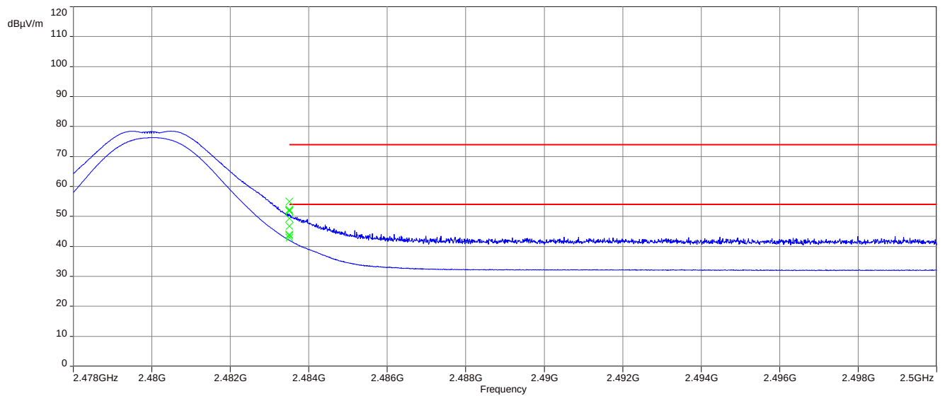
Plot 3: Upper restricted band, 2480 MHz (internal antenna setup)
