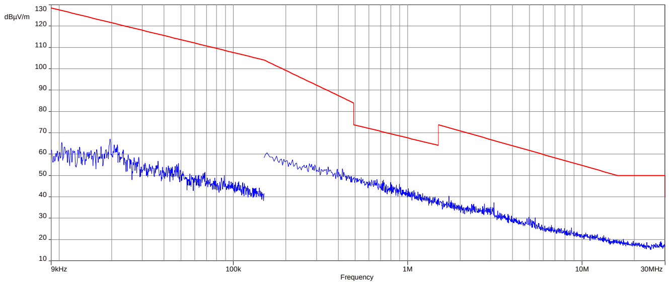
Plot 1: 9 kHz to 30 MHz, 2405 MHz, transmit mode (internal antenna setup)
