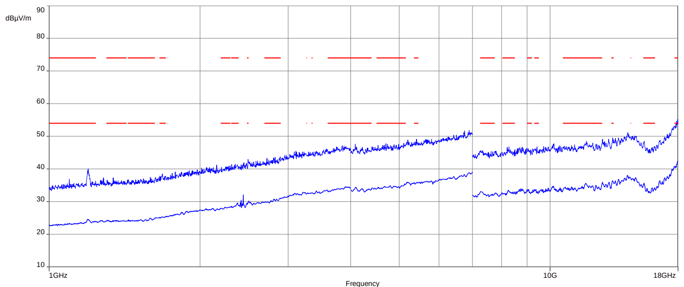
Plot 2: 1 GHz to 18 GHz, TX mode, 2440 MHz, vertical & horizontal polarization (internal antenna setup)
