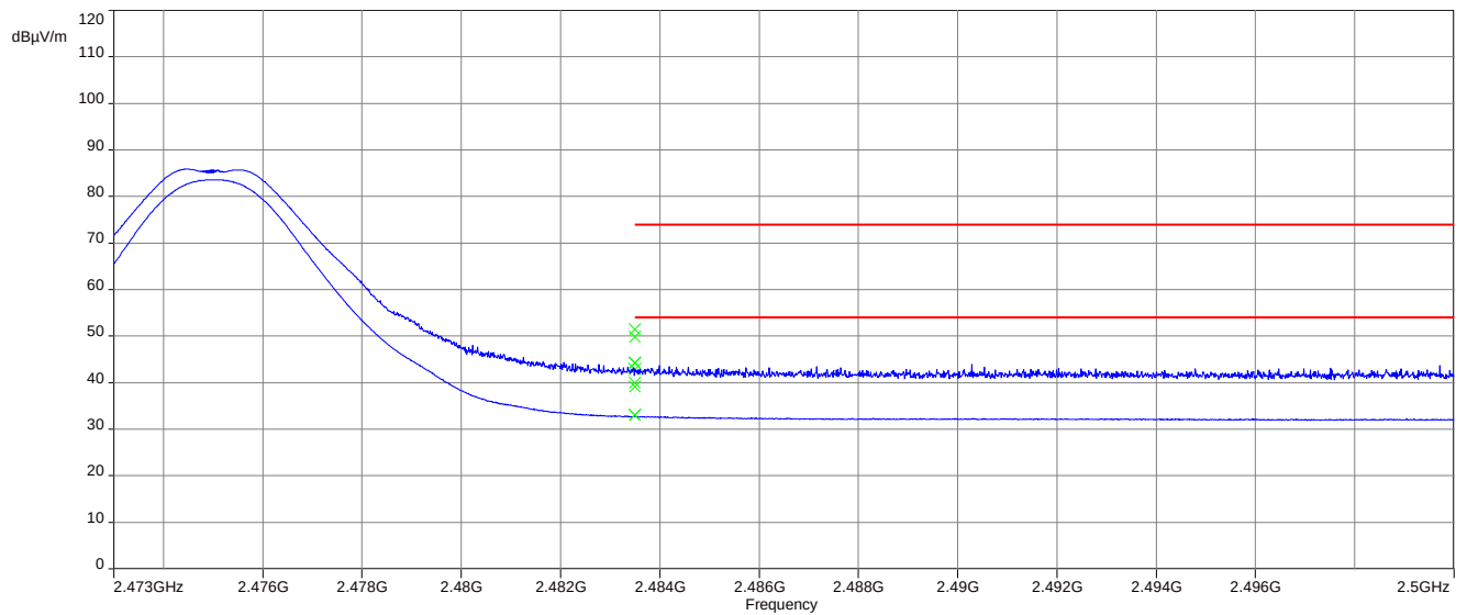
Plot 5: Upper restricted band 2475 MHz (external antenna setup)
