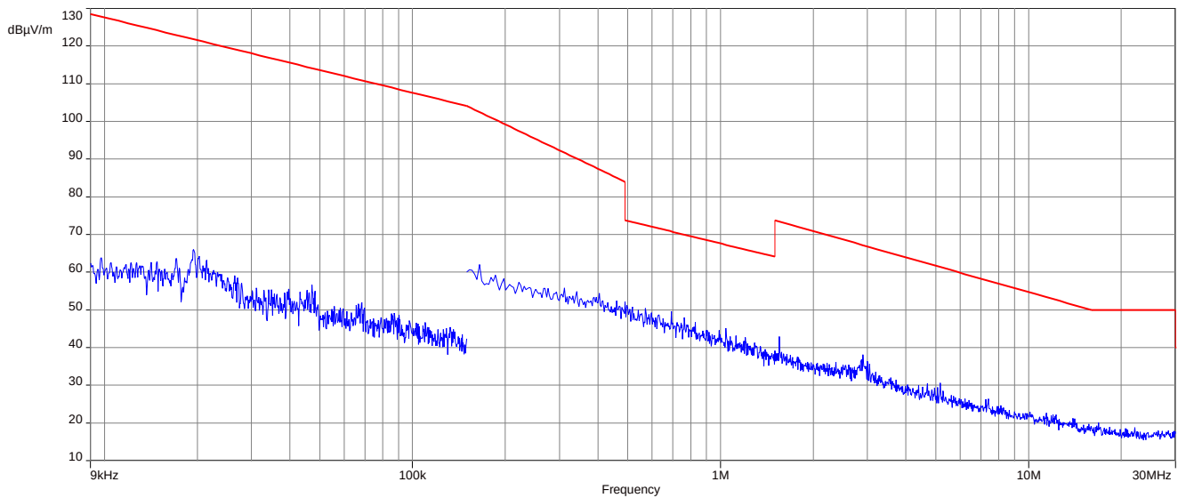
Plot 5: 9 kHz to 30 MHz, 2440 MHz, transmit mode (external antenna setup)
