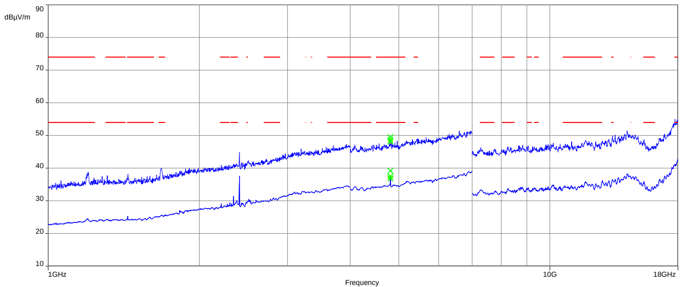
Plot 5: 1 GHz to 18 GHz, TX mode, 2405 MHz, vertical & horizontal polarization (external antenna setup)
