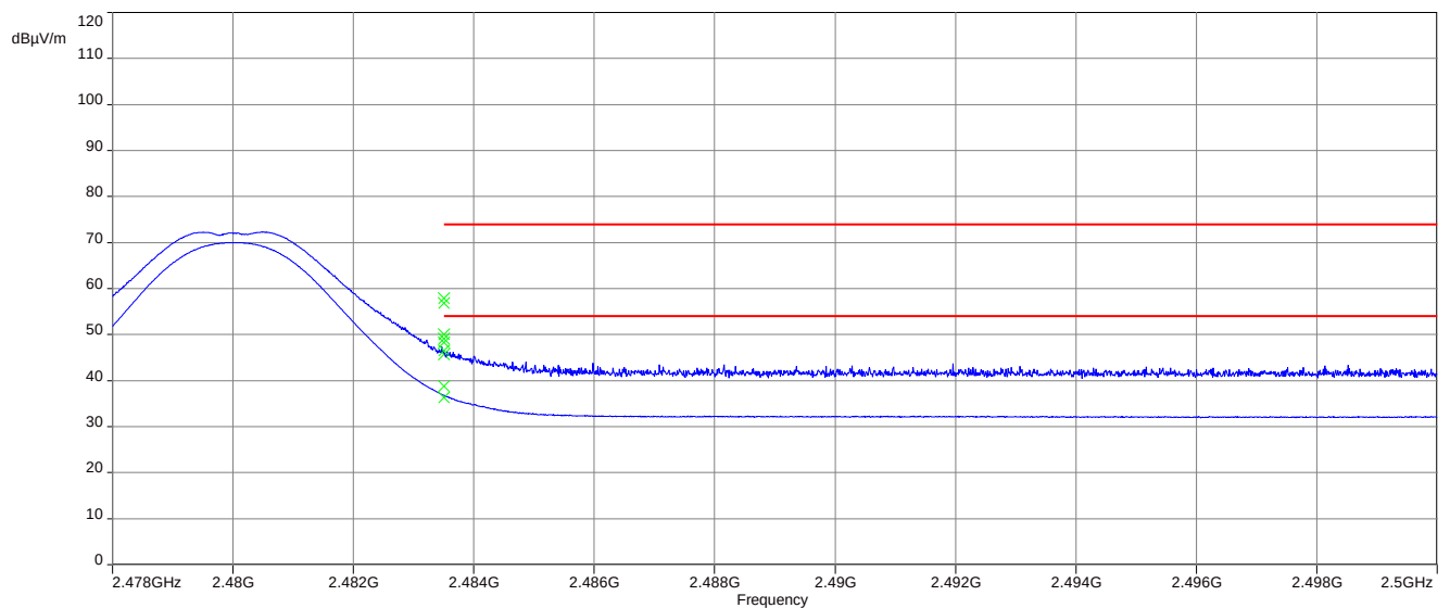
Plot 6: Upper restricted band 2480 MHz (external antenna setup)
