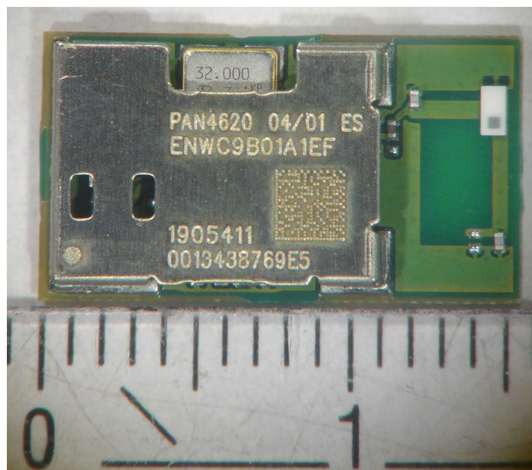
Photo 2: Module PCB, front side view
