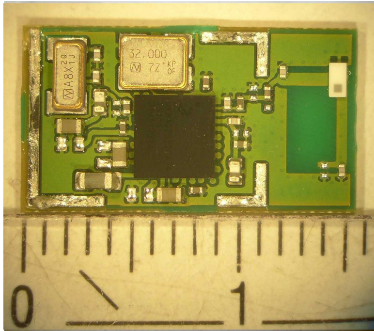
Photo 3: Module PCB, front side view (shielding removed)
