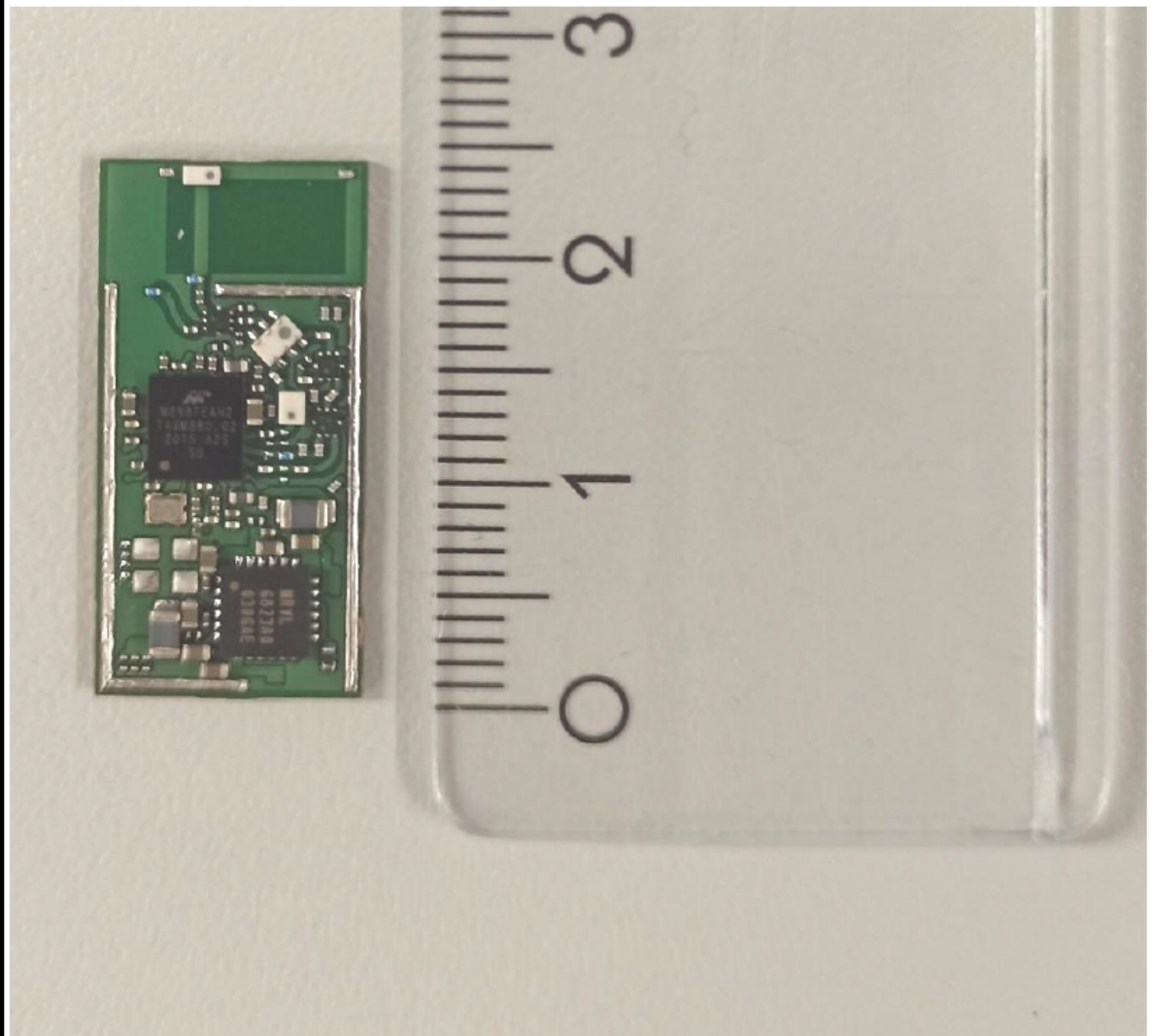
ENWF9408A1EF_top_nocase
