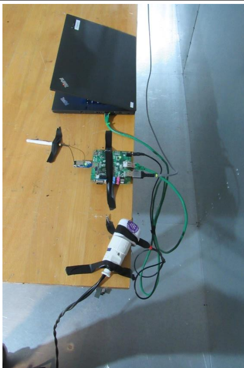
Setup for measurements 150 kHz - 30 MHz (2)
