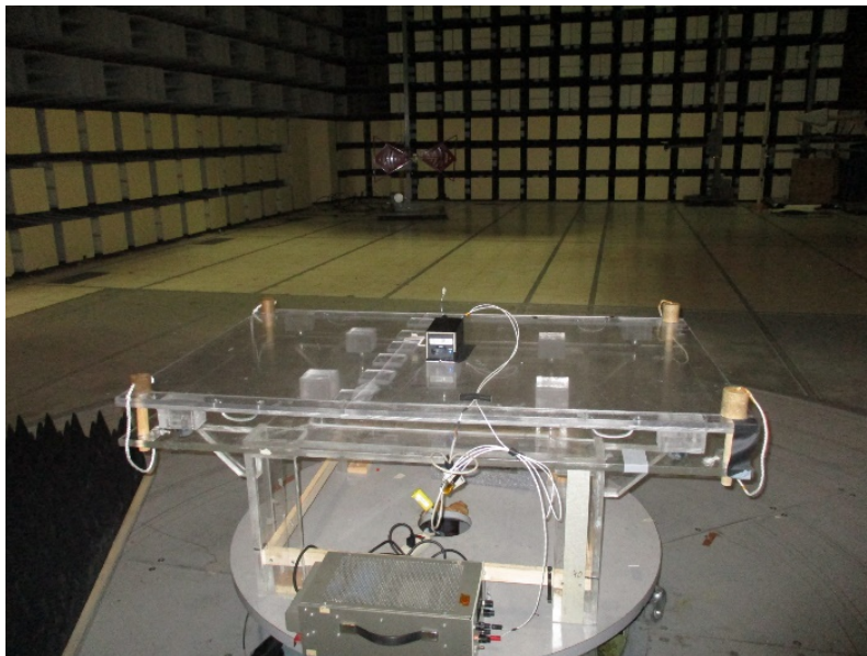
Radiated Emissions, 30MHz to 1 GHz
