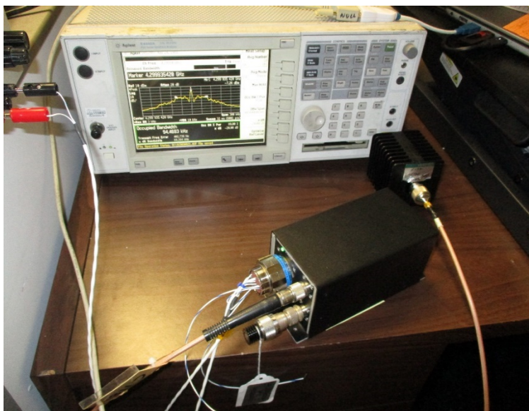
Conducted Antenna Port Measurements: Power, Bandwidth, OBW, Spurious
