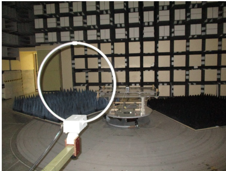
Radiated Emissions, 9kHz – 30MHz
