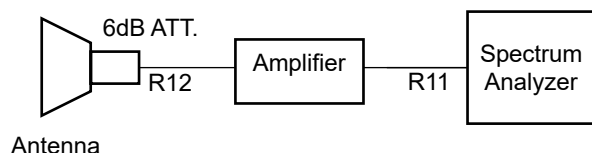
Diagram of the measurement instruments ( 1000 - 2000 and 3000 - 18000 MHz )
