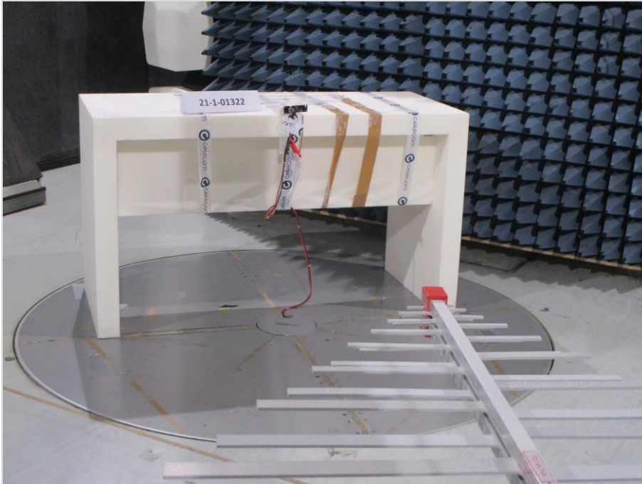
Photograph 3: EUT Test Setup in the semi anechoic chamber, Electric Field Strength
