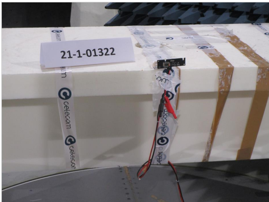
Photograph 2: EUT Test Setup in the semi anechoic chamber, Electric Field Strength
