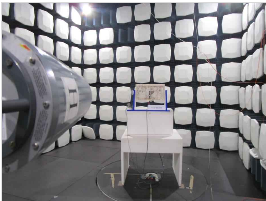
Photograph 4: EUT Test Setup in the fully anechoic chamber, Electric Field Strength
