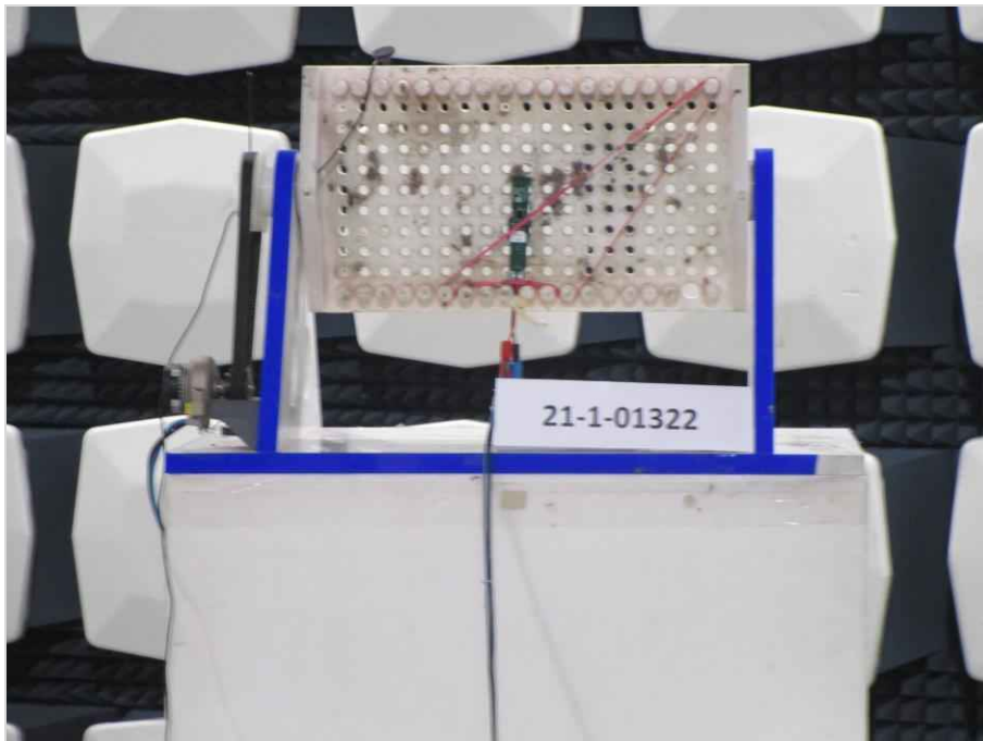
Photograph 3: EUT Test Setup in the fully anechoic chamber, Electric Field Strength
