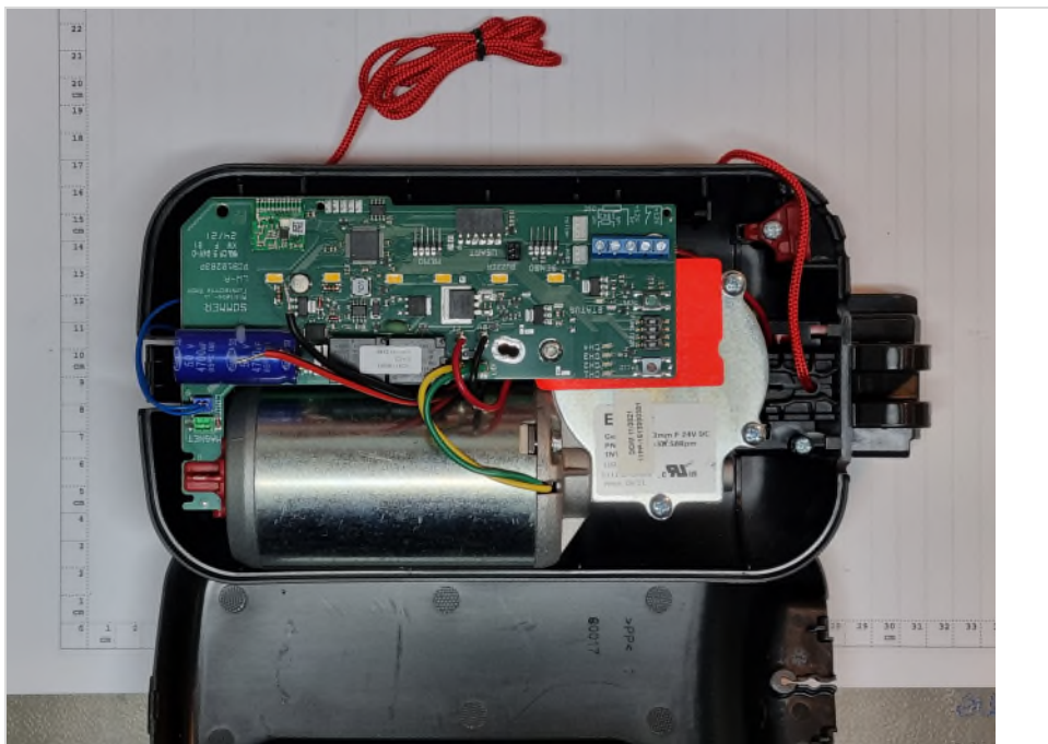
Photograph 2: EUT 1_Top side view_internal
