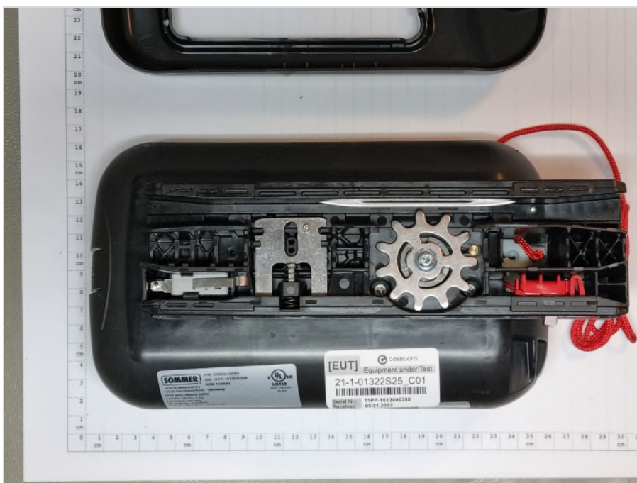
Photograph 8: EUT 2_Bottom side view
