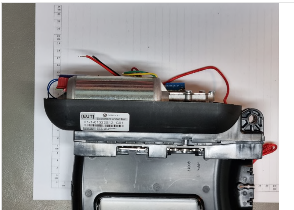
Photograph 4: EUT 1_Left side view
