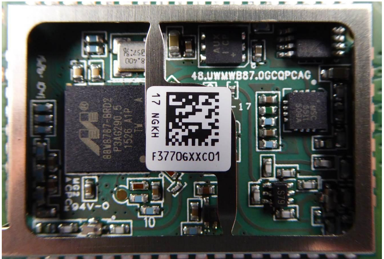
160090_40. jpg: EUT – Main Unit – Shielded Unit close up
