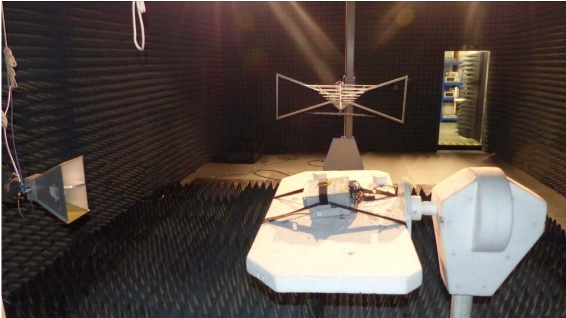
Photo 5: Radiated test setup for 1GHz – 25GHz
