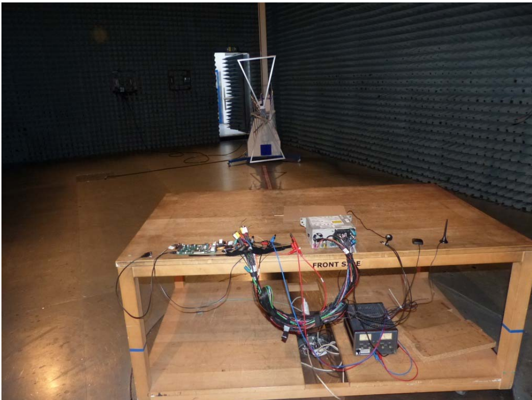
Photo 4: Radiated test setup for 30MHz – 1 GHz.
