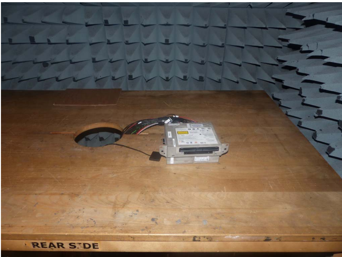
Photo 2: Radiated test setup for H-Field
