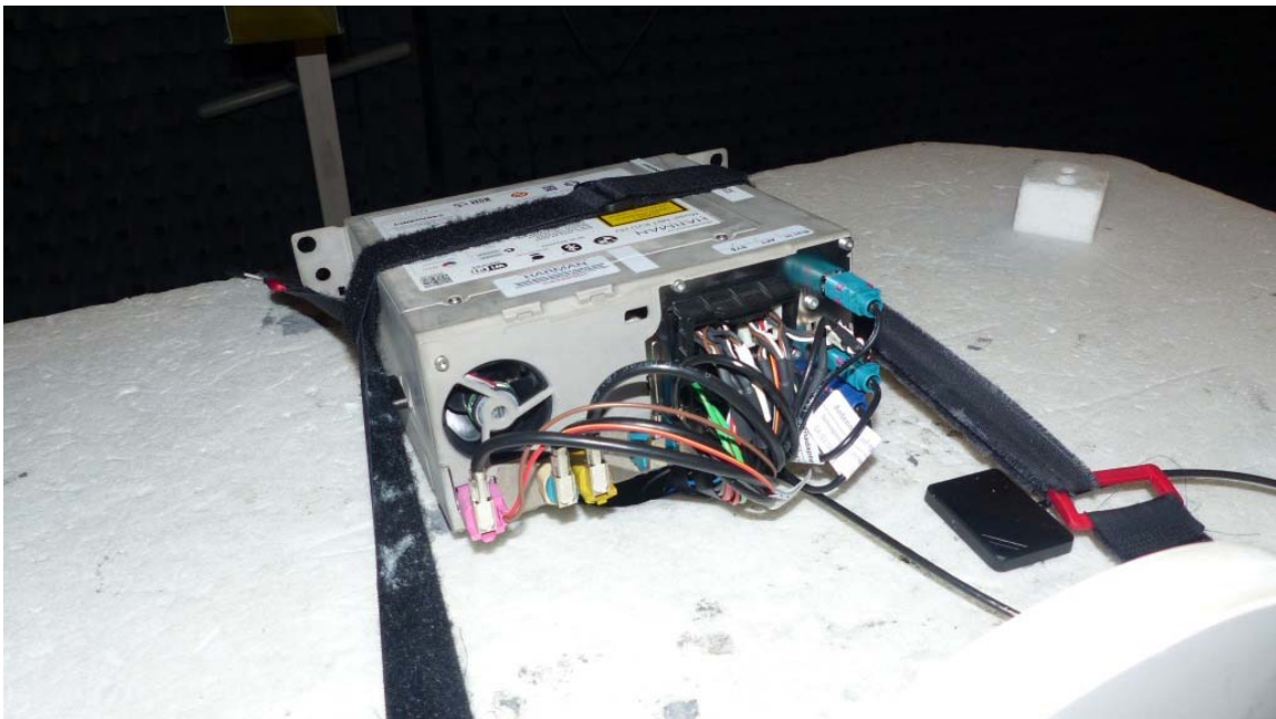
Photo 6: Radiated test setup for 1GHz – 25GHz
