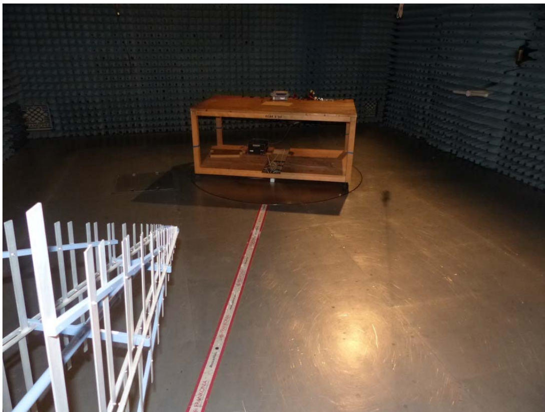
Photo 3: Radiated test setup for 30MHz – 1 GHz.
