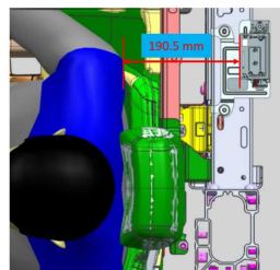
Picture left: Minimum distance of 190mm between GSM/UMTS/LTE-Ant. and passenger Picture right: Minimum distance of 95mm between WLAN Antenna and passenger
