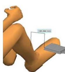
Picture left: Minimum distance of 190mm between GSM/UMTS/LTE-Ant. and passenger Picture right: Minimum distance of 95mm between WLAN Antenna and passenger
