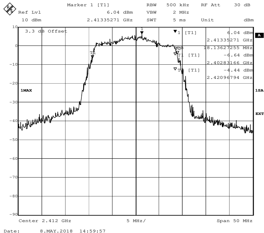
WLAN mode n, low channel
