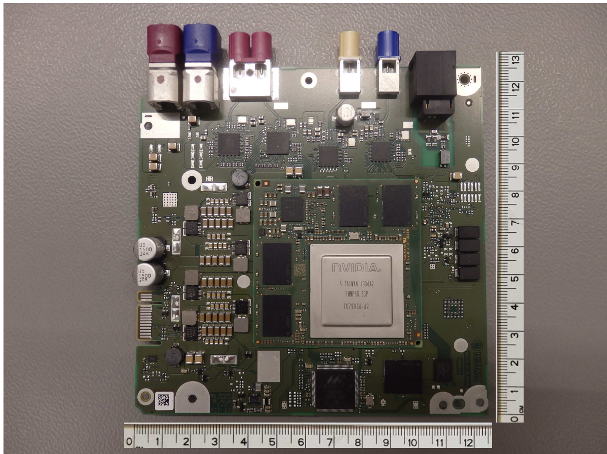
PCBA_MMB_3860442 top / bottom (125 x 125 mm)
