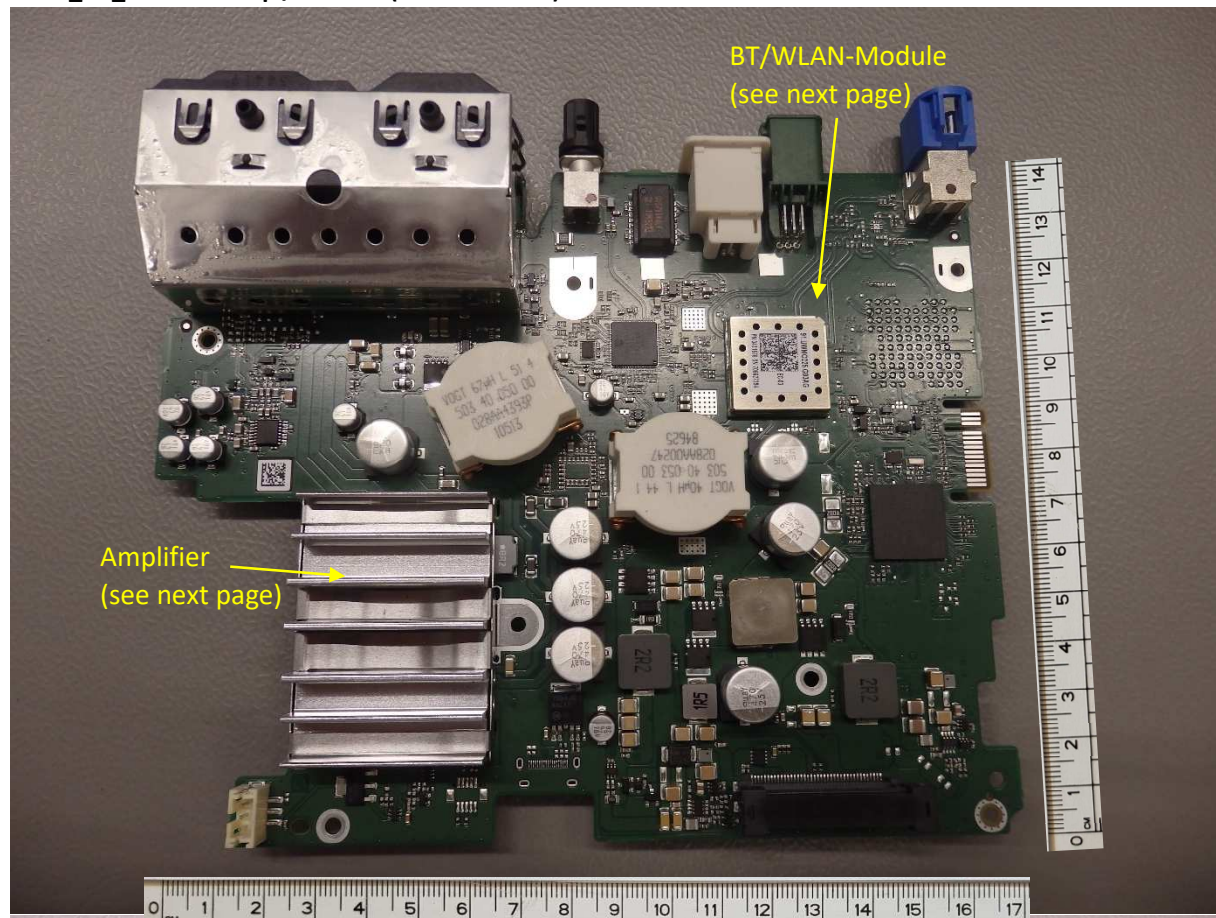
PCBA_BB_3899608 top / bottom (168 x 136 mm)
