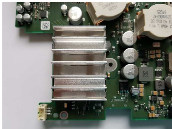
Heat Sink mounted
