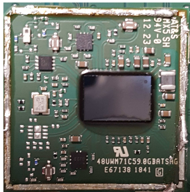
without shielding plate
