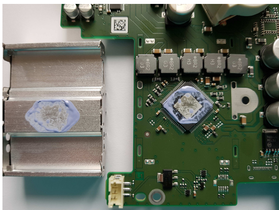
Heat Sink & Power amplifier
