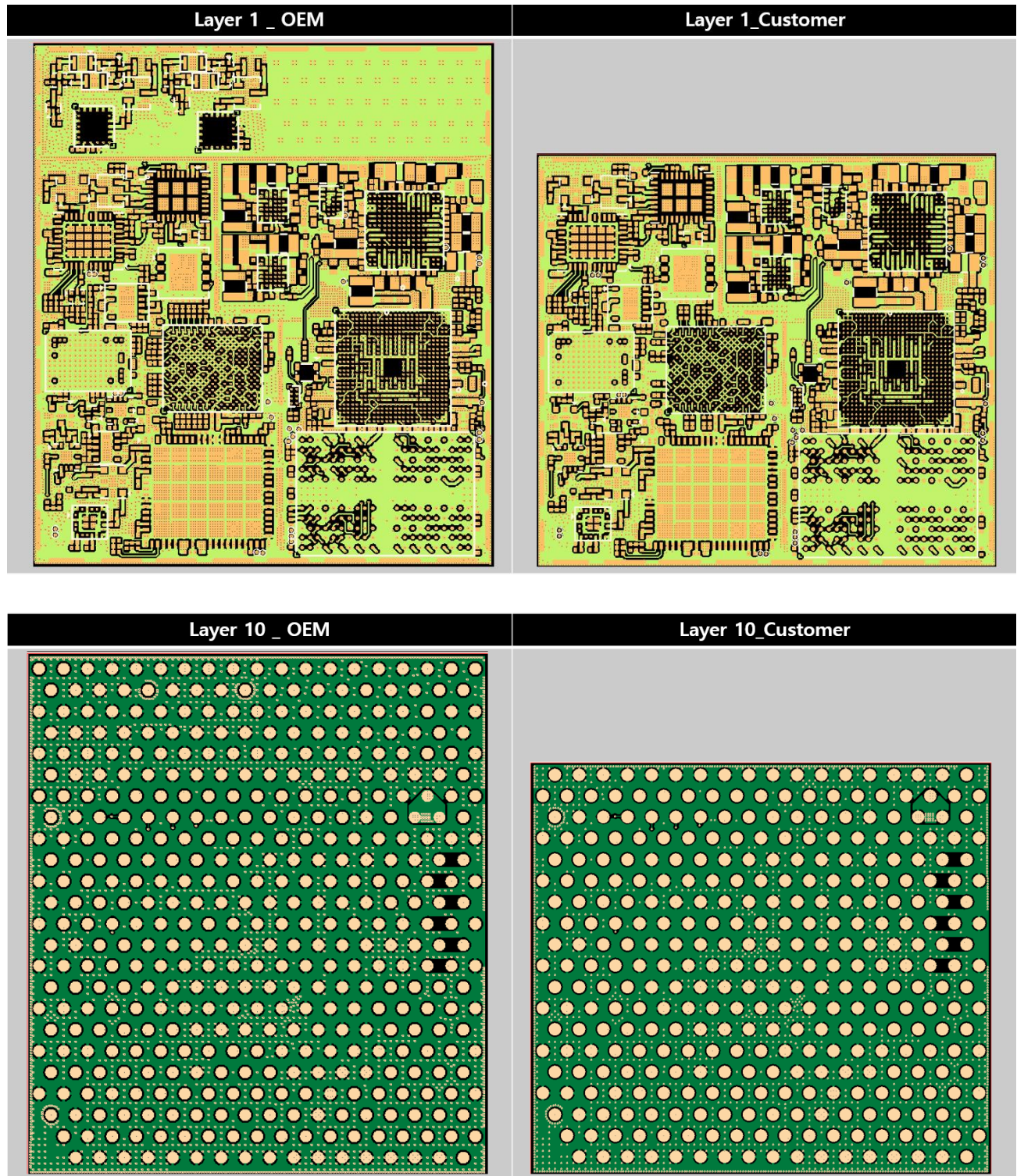
Figure 1.2 : layout comparison
