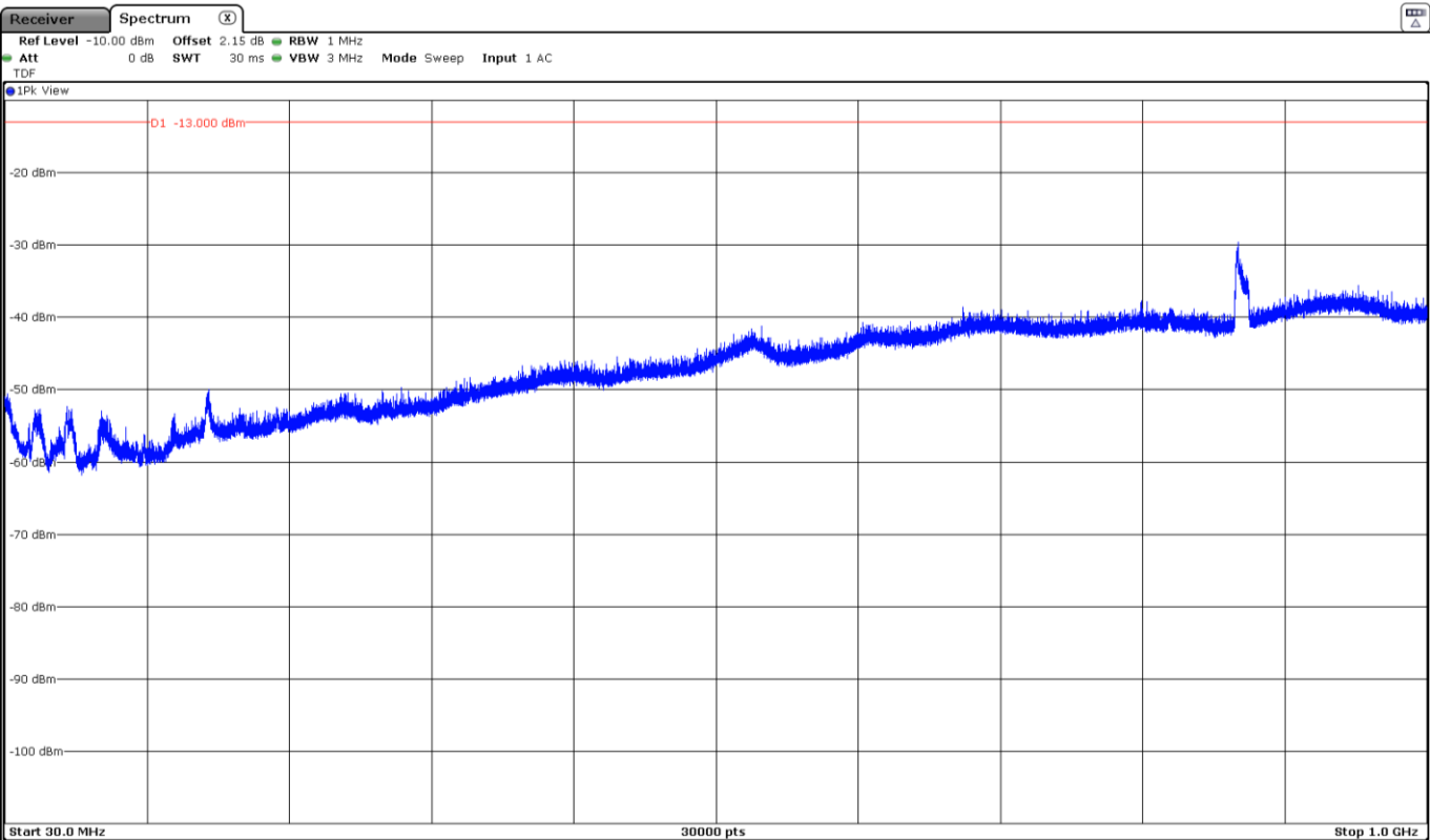
The peak at 874MHz corresponds to the LTE signal downlink of DC_5A_n66A.
