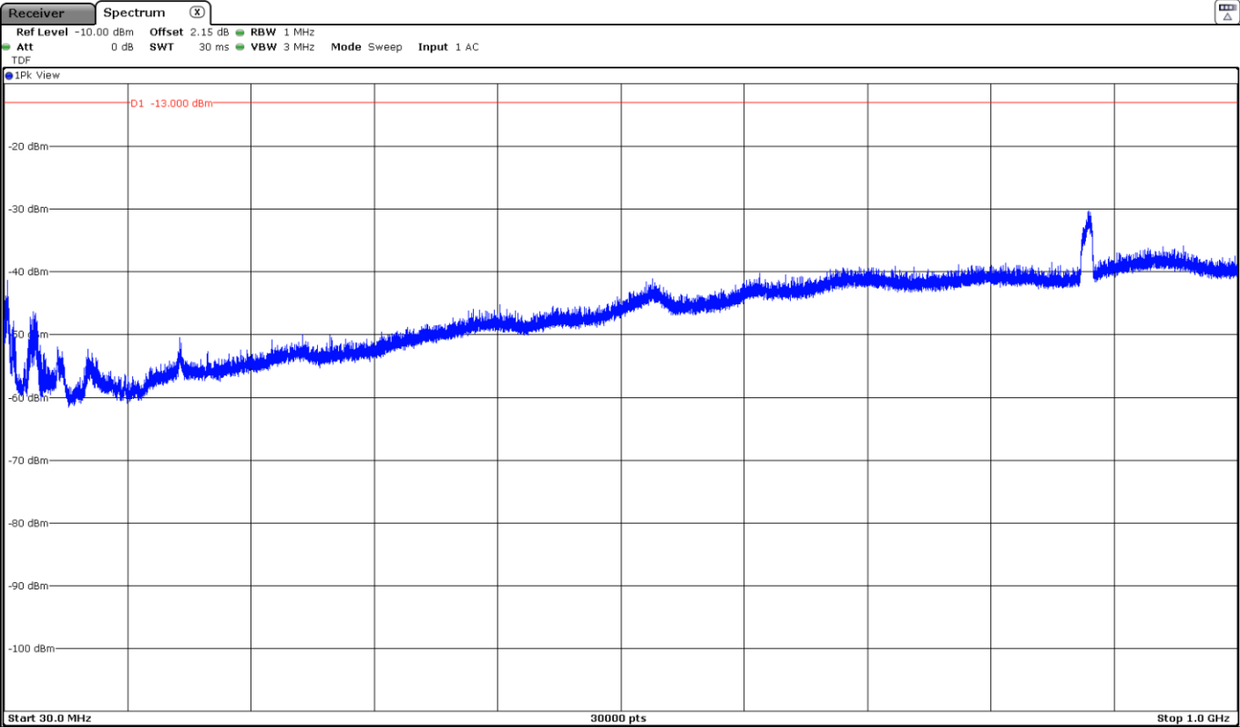
The peak at 881.5MHz corresponds to the LTE signal downlink of DC_5A_n66A.
