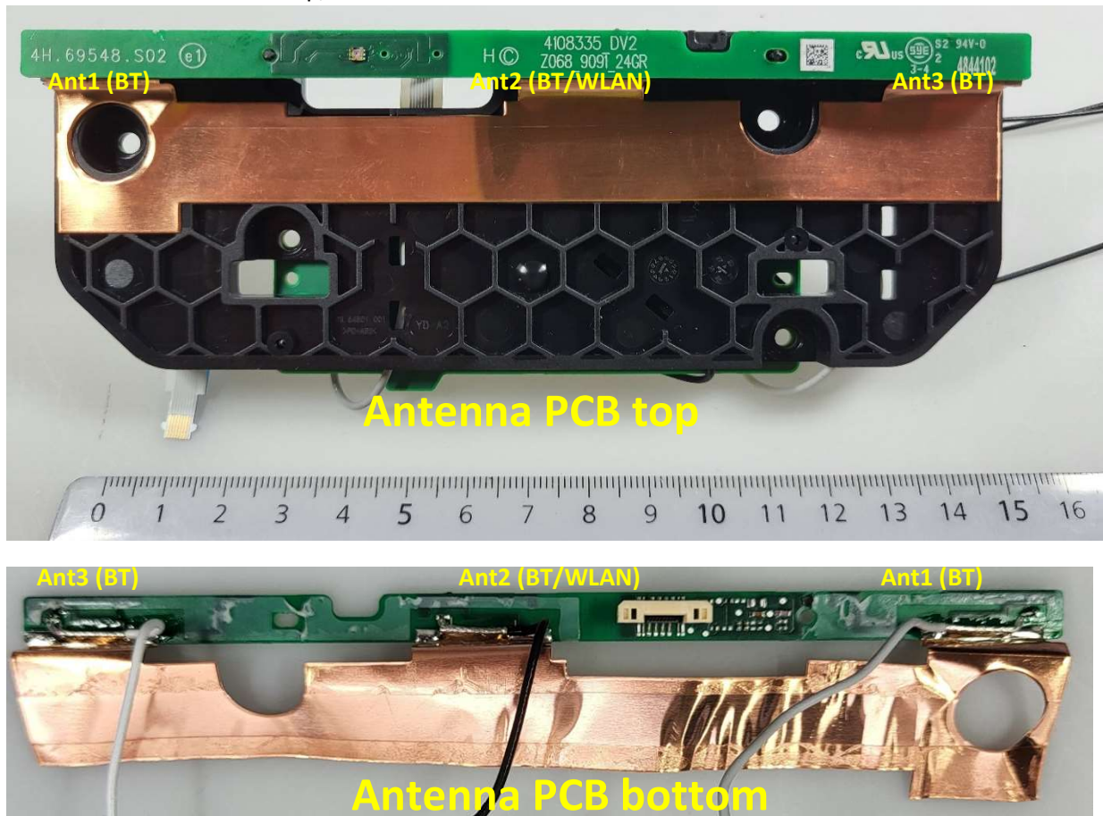
PCBA Z068 9091 Antenna top/bottom
