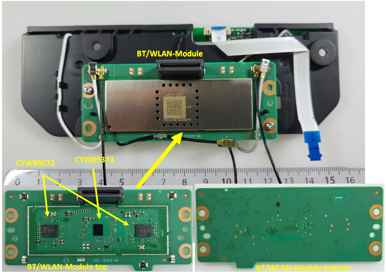
PCBA Z068 5070 top/bottom
