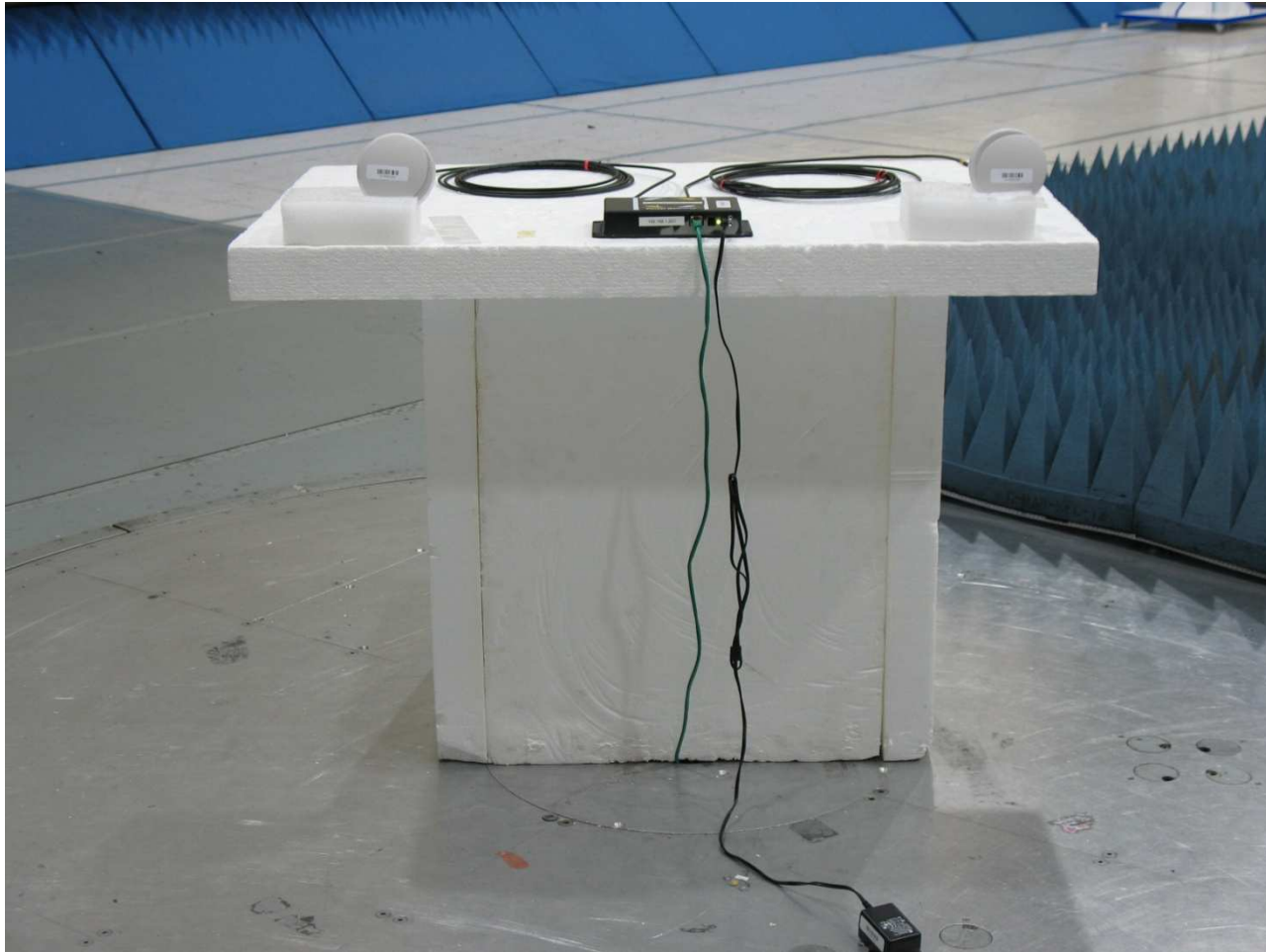
Radiated Spurious Emissions - MC2400PTMSMA Antenna
