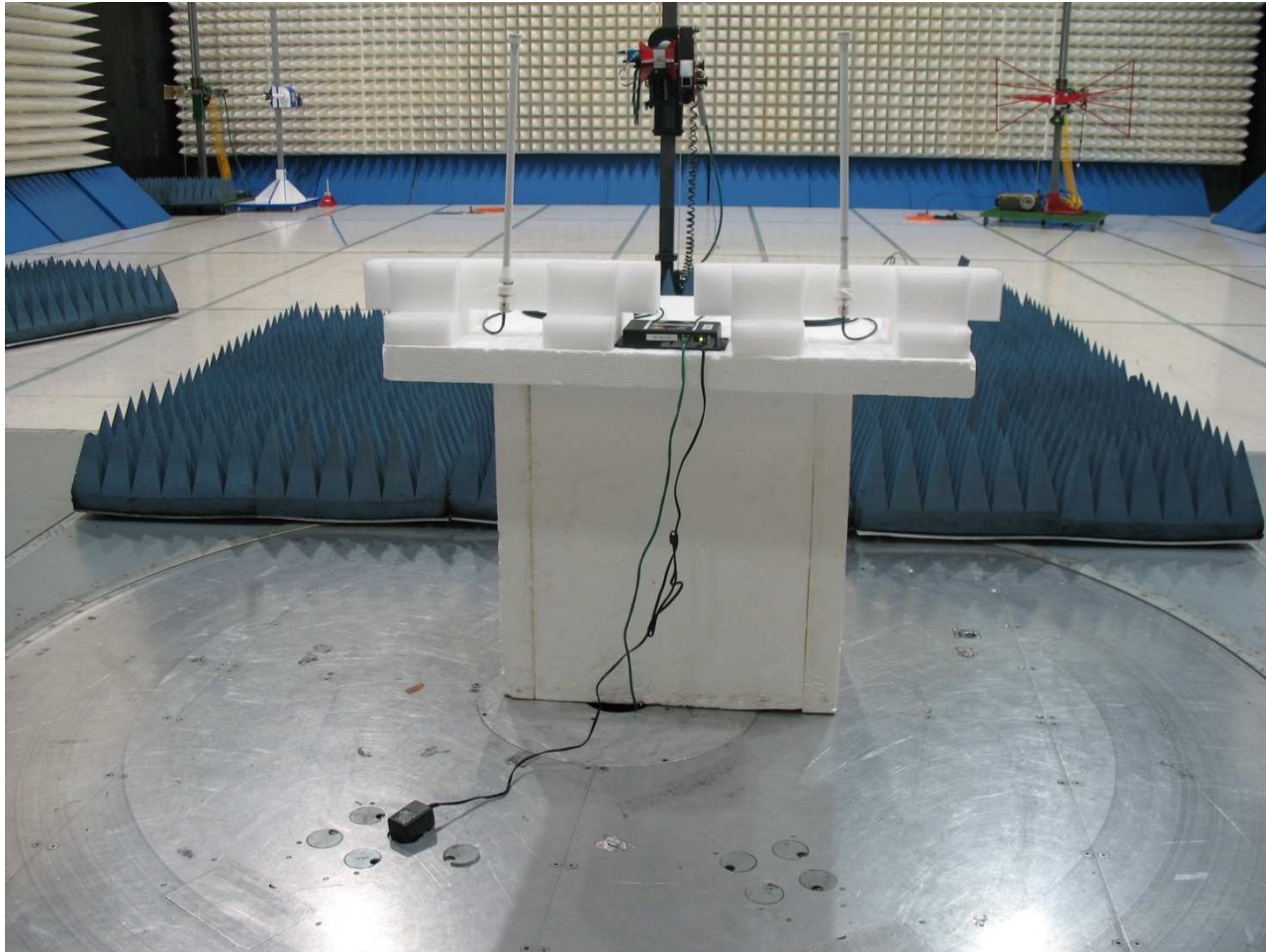
Radiated Spurious Emissions - BS2400XL3 Antenna
