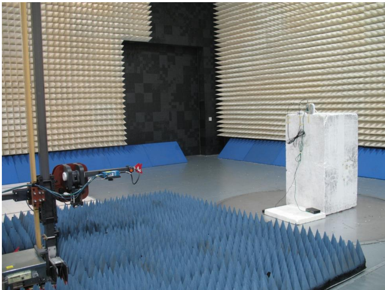
Radiated Spurious Emissions, 1GHz-40GHz, PCTEL (Maxrad) MC2400PTMSMA Ceiling Mount Antenna
