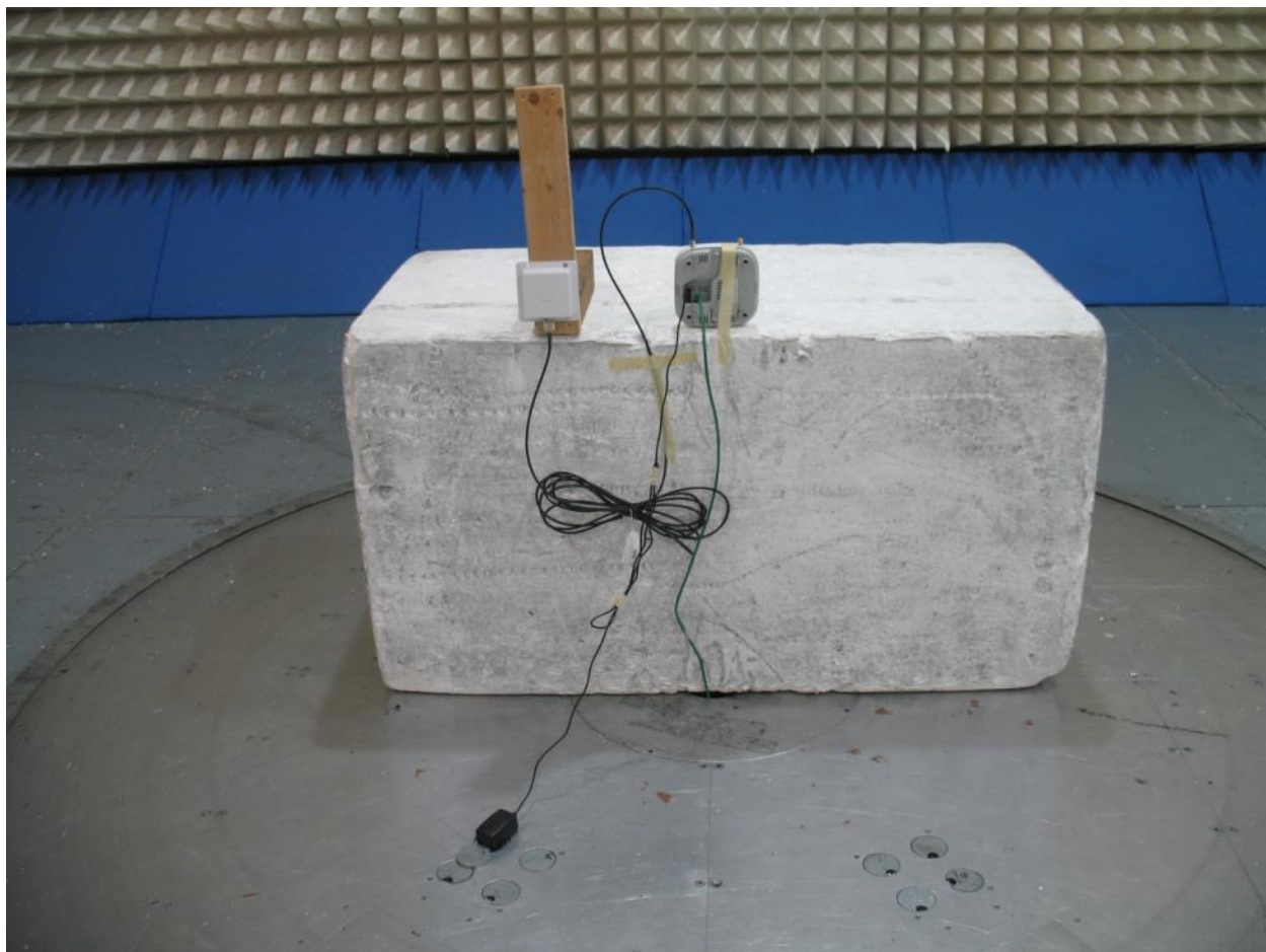
Setup - Mobile Mark (Comtelco) CMTB36247V Wall Mount Antenna
