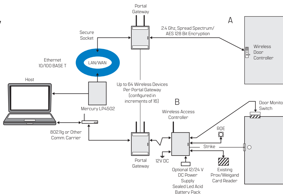
Figure 2 Hardware Overview
