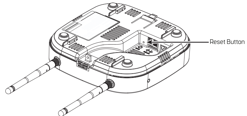
Figure 11 Wi-Fi Reset Button
