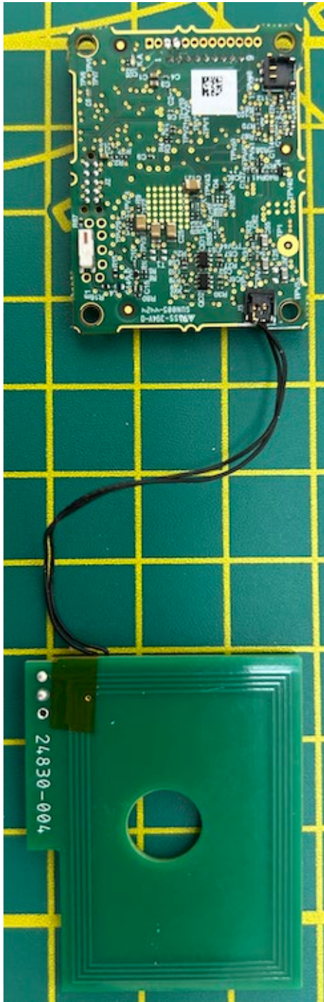
CSM-200 Module Connected to HD Antenna
