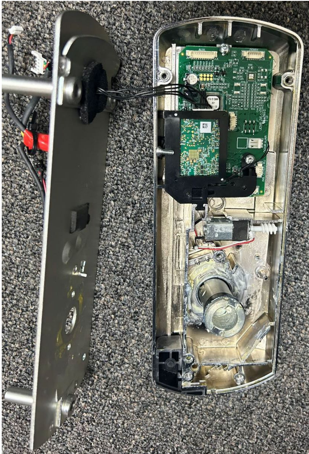
PCBs and Door Plate
