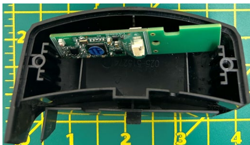
Host's Certified Zigbee TX Endcap – Back View
