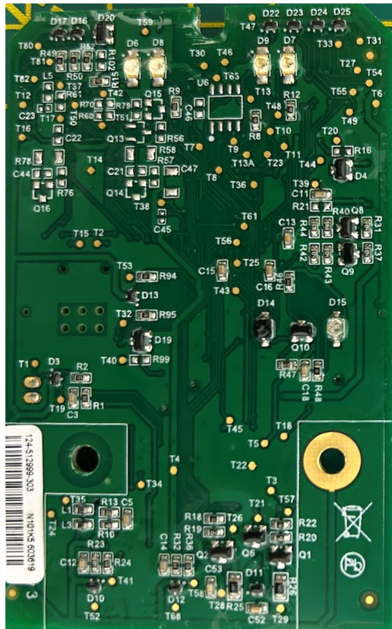
Host E7900 PCB – Back View
