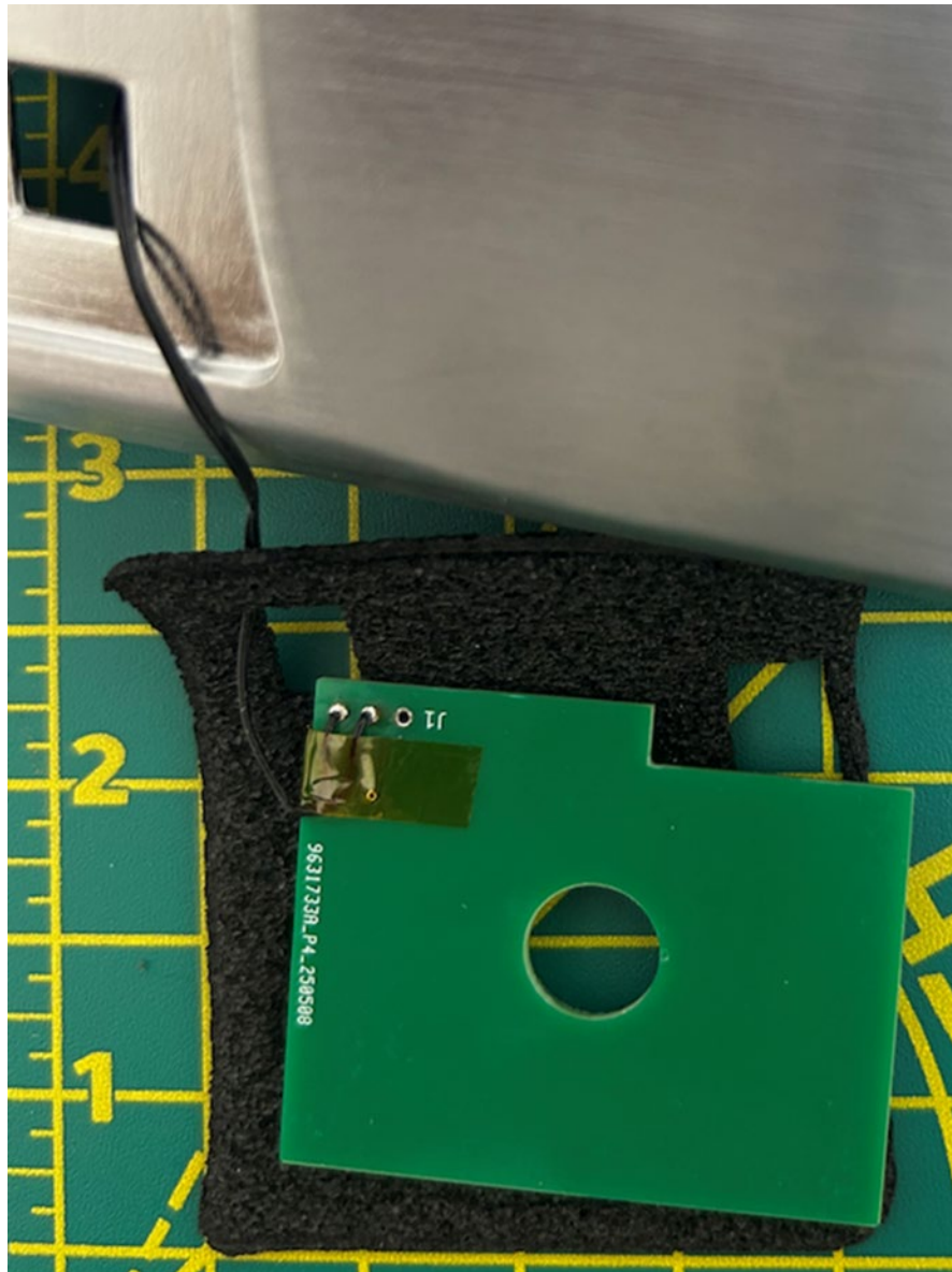
HF Antenna Connector to HF Antenna; for placement in recessed area on door lock exterior
