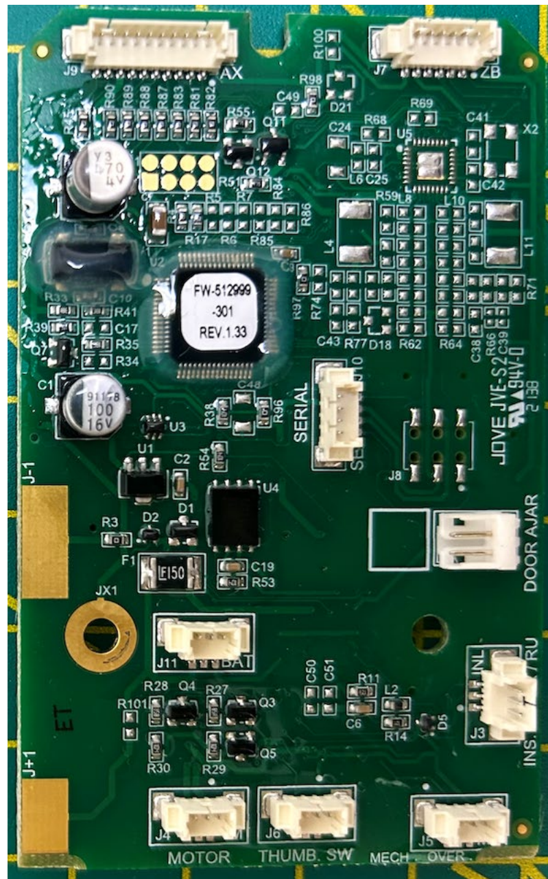
Host E7900 PCB – Front View
