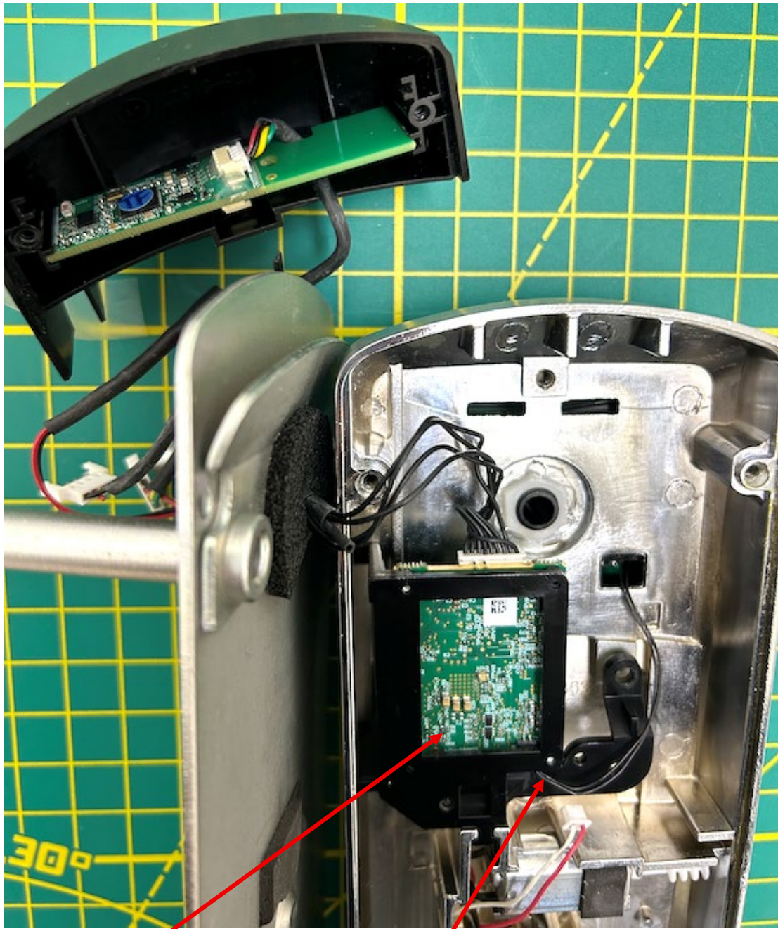
CSM-200 Module HF Antenna Connector Wire to HF Antenna (not visible)
