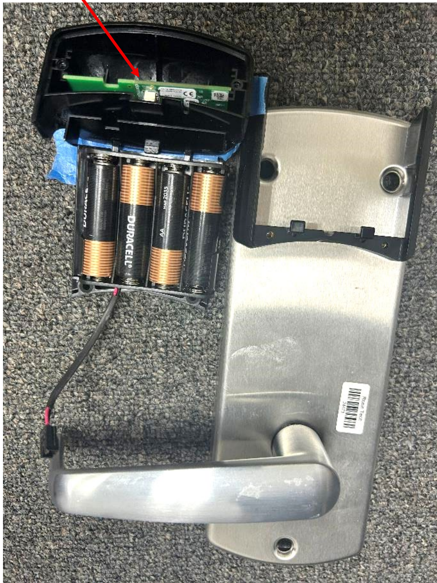
Host's Certified Zigbee TX in Endcap and Battery Cage
