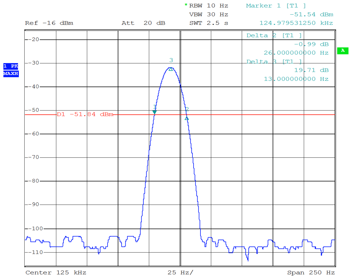
Plot 1, 20dB Bandwidth
