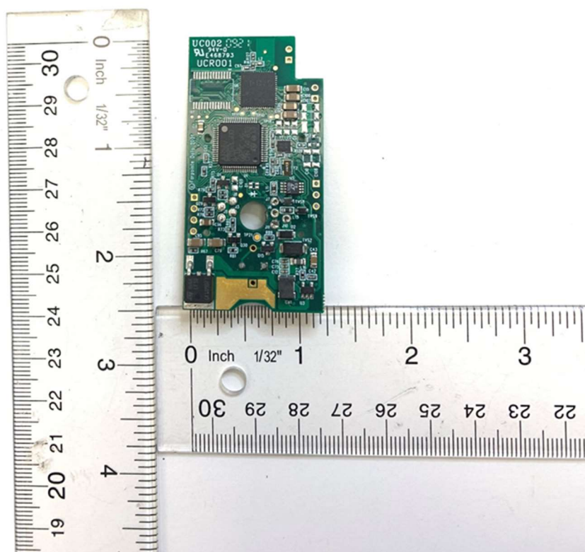
RF Board Front - Farpointe Data, Inc. Confidential & Proprietary Information
