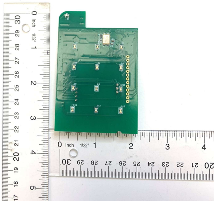
Keypad Controller Board Front - Farpointe Data, Inc. Confidential & Proprietary Information
