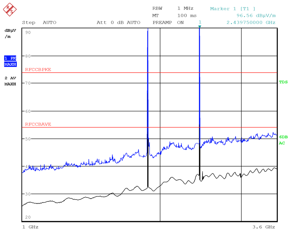
Figure 8.1-11: Radiated spurious emissions with GSM 1900 at mid channel and BLE at mid channel – antenna in horizontal polarization
